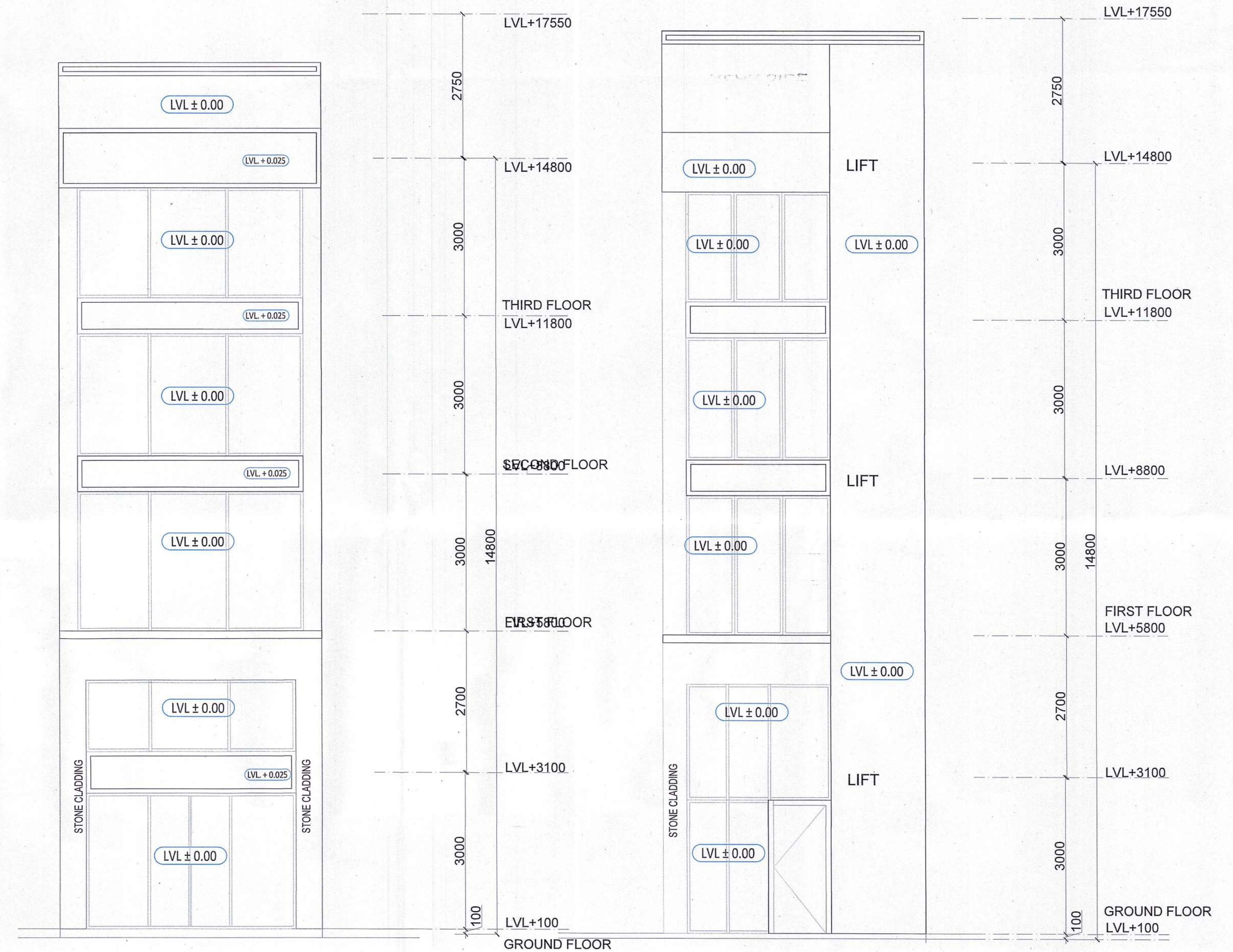
REAR SIDE ELEVATION
