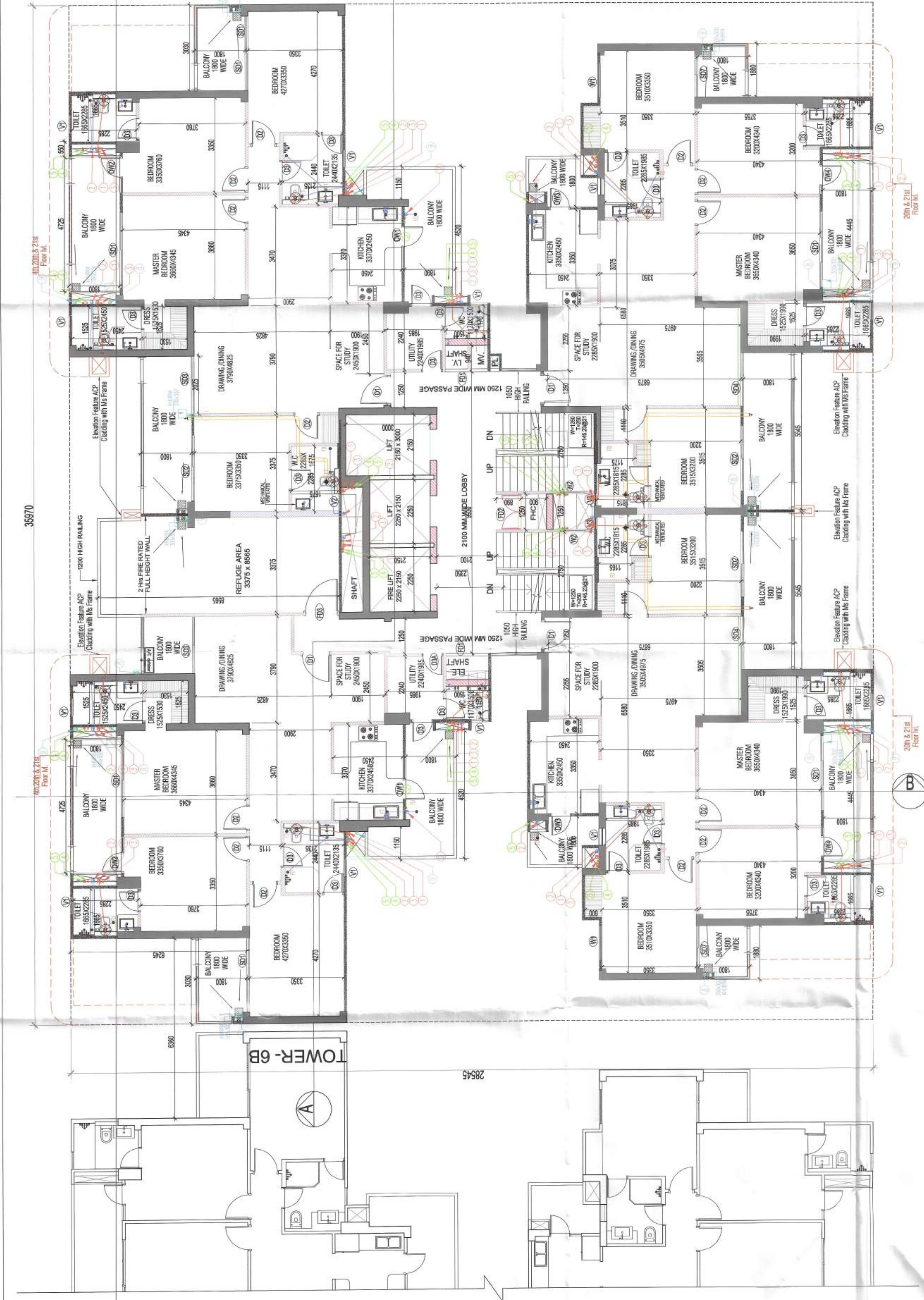
TOWER-6C REFUGE FLOOR PLAN (20TH &amp; 30TH LVL PLAN) (FFL + 61850 &amp; + 92350)
