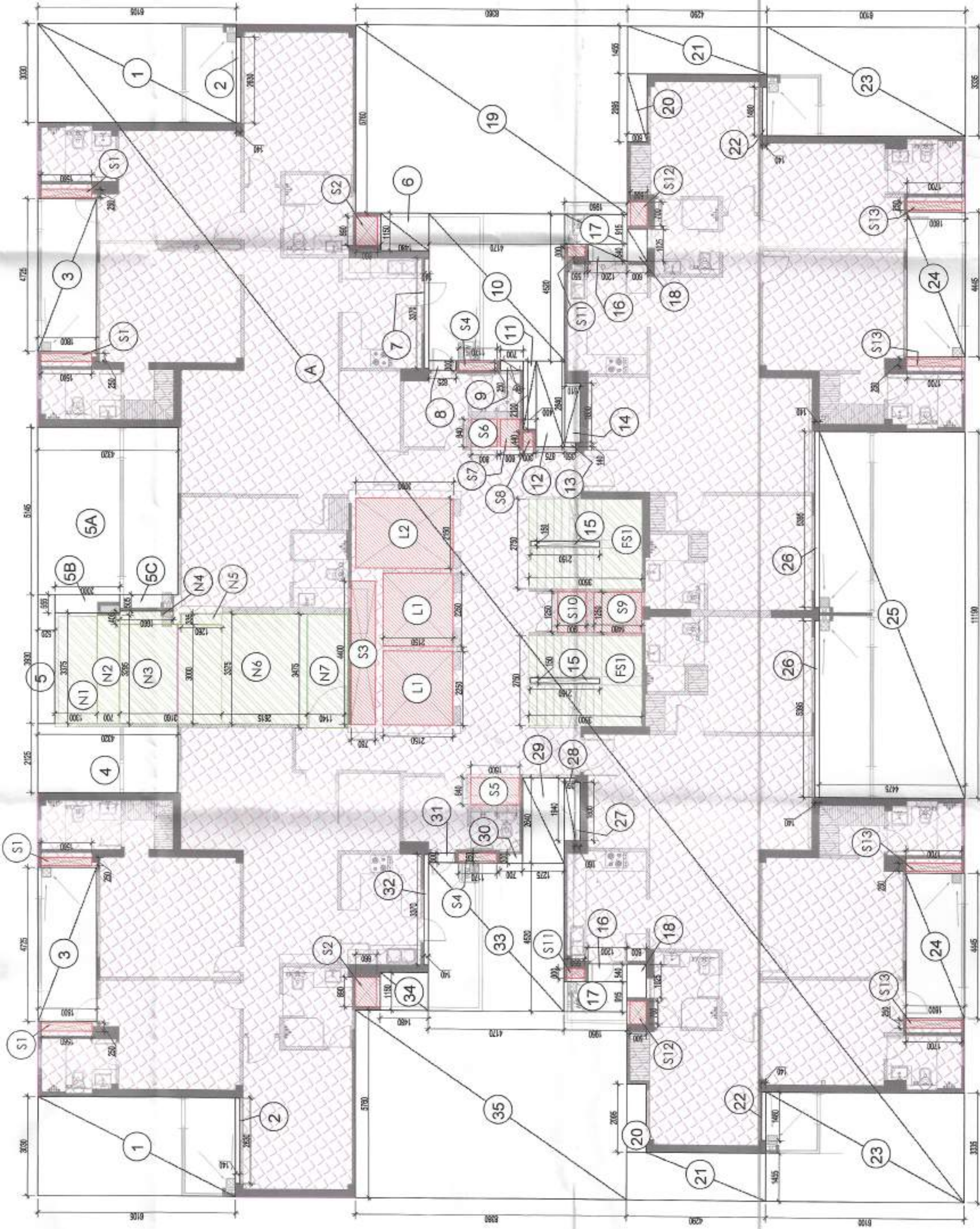
TOWER-6C 20TH & 30TH LVL AREA DIAGRAM (REFUGE FLOOR)
