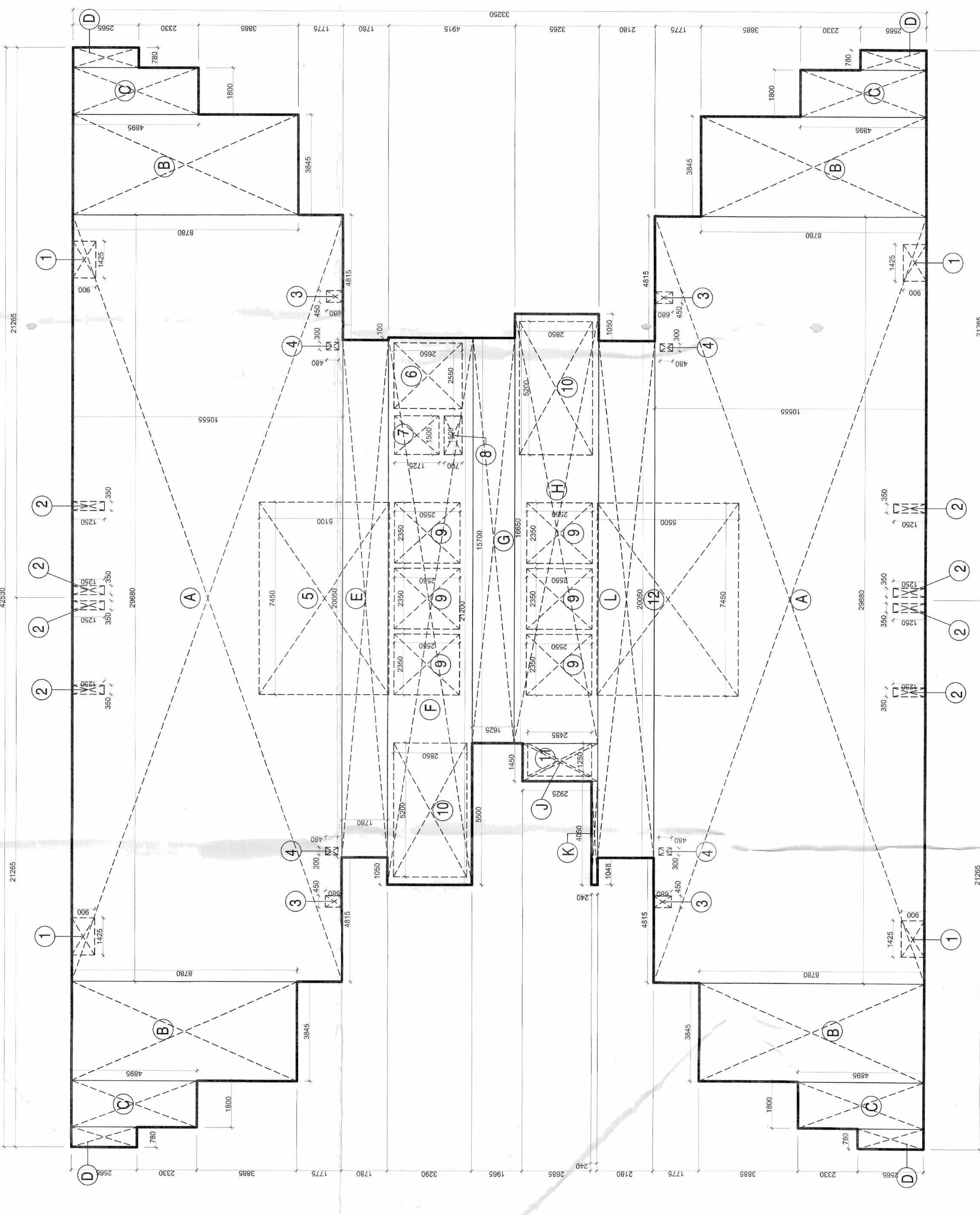
TOWER-27 TYPICAL FLOOR PLAN AREA DIAGRAM
