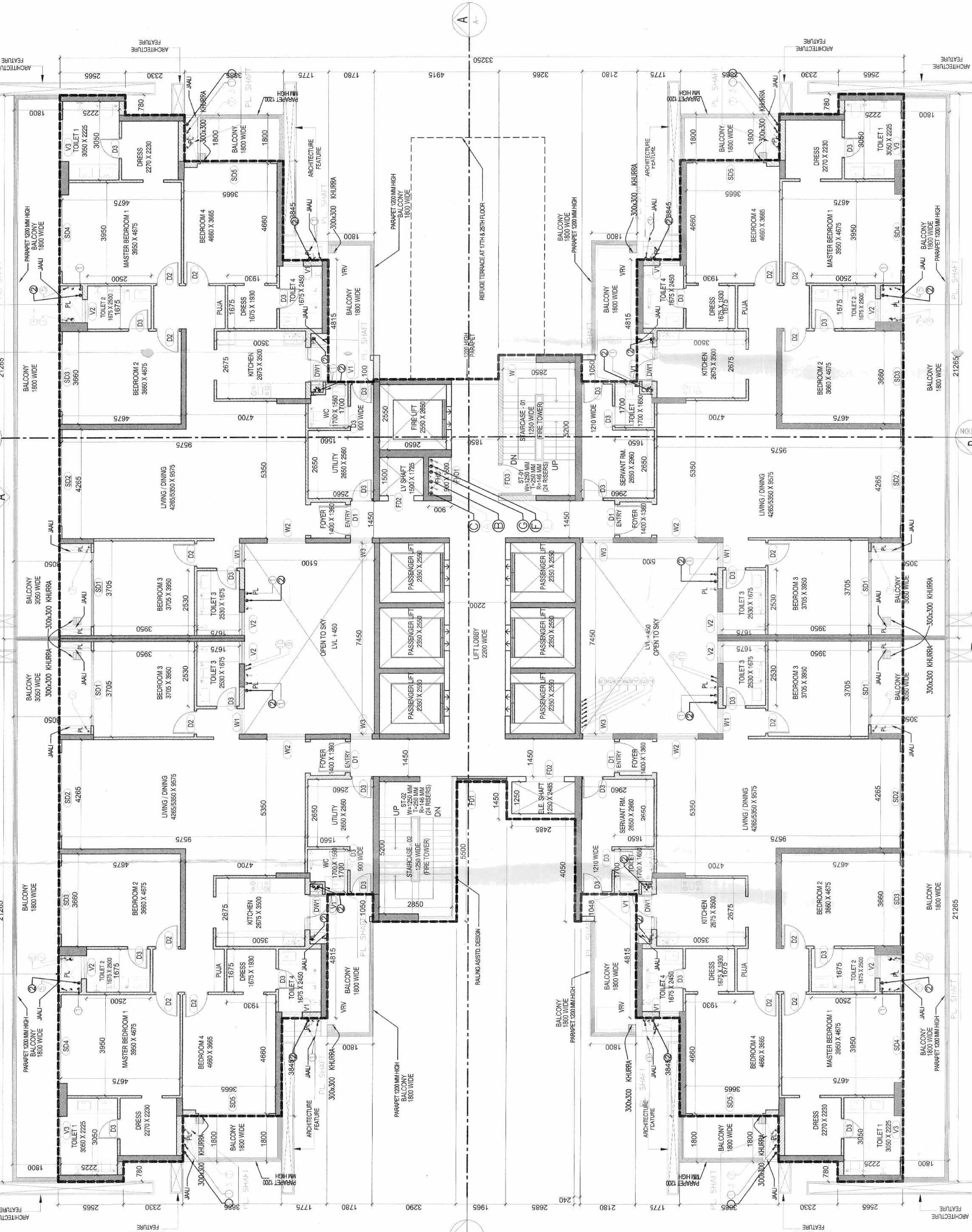
TOWER 27 - TYPICAL FLOOR PLAN (2nd to 32st excluding 17th and 25th) TOILET DETAIL-TYPICAL
