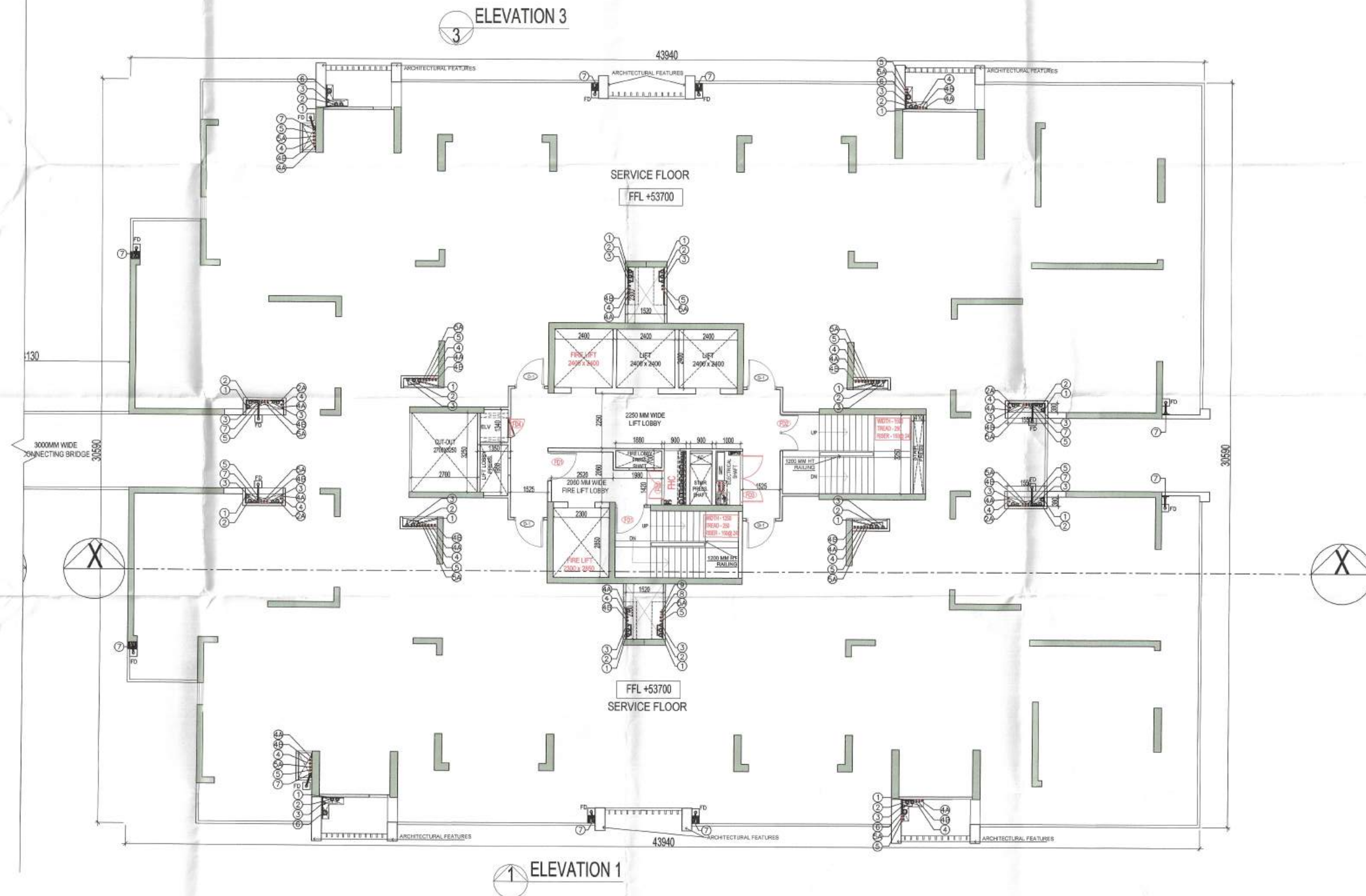
14th FLOOR (SERVICE FLOOR) PLAN TOWER- C
