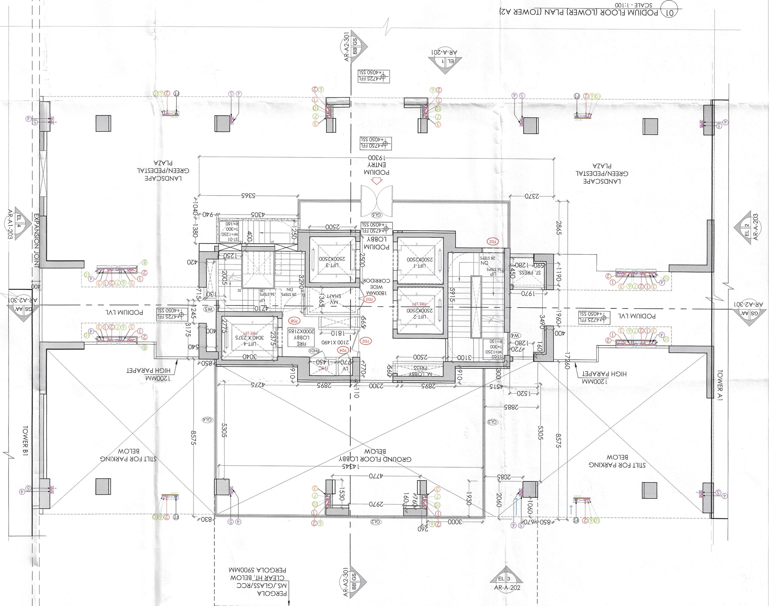
01. PODIUM FLOOR (LOWER) PLAN (TOWER A2)
