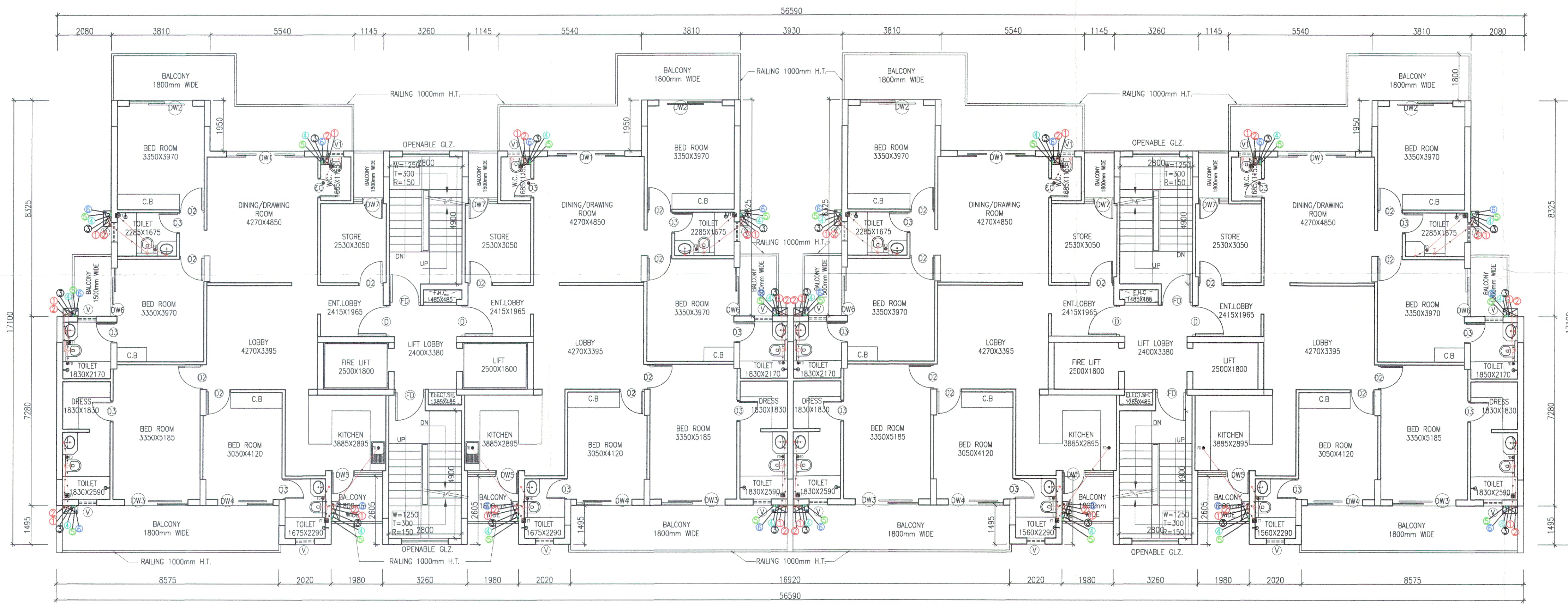
TYP. FLOOR PLAN (2ND TO 4TH) (BLOCK - 9, 10 & 11)
