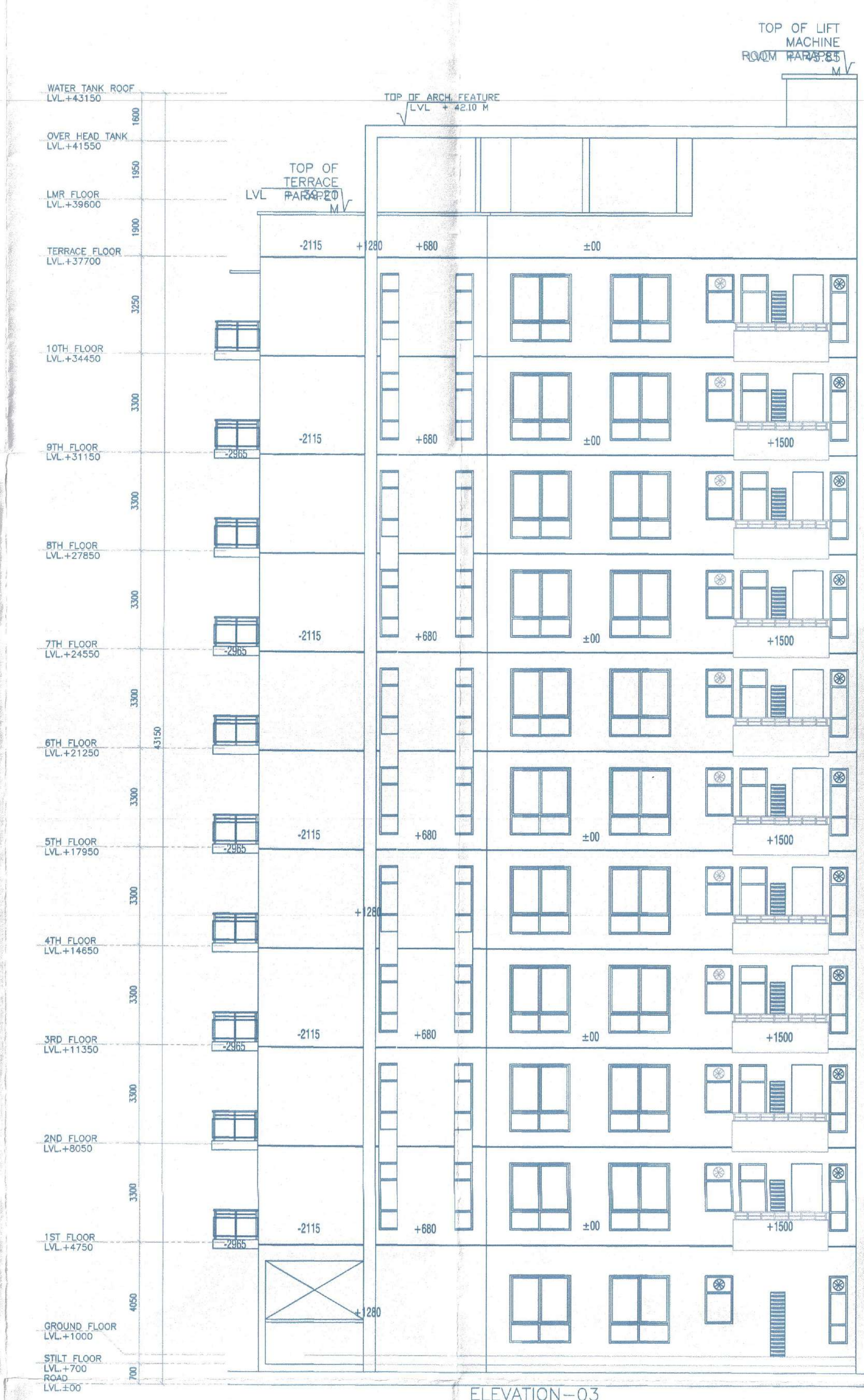
ELEVATION-03 BLOCK-J
