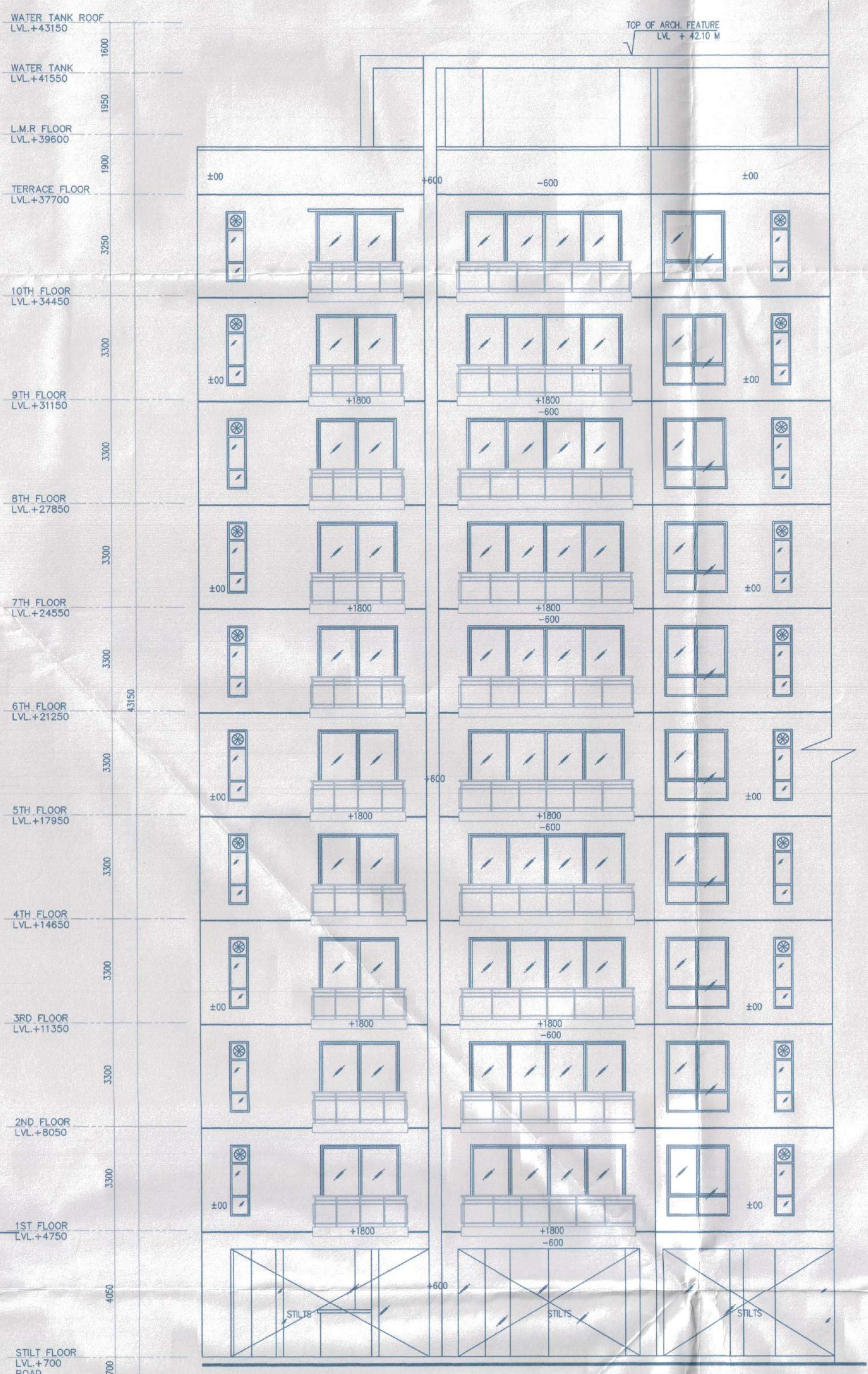
ELEVATION-01 BLOCK-K
