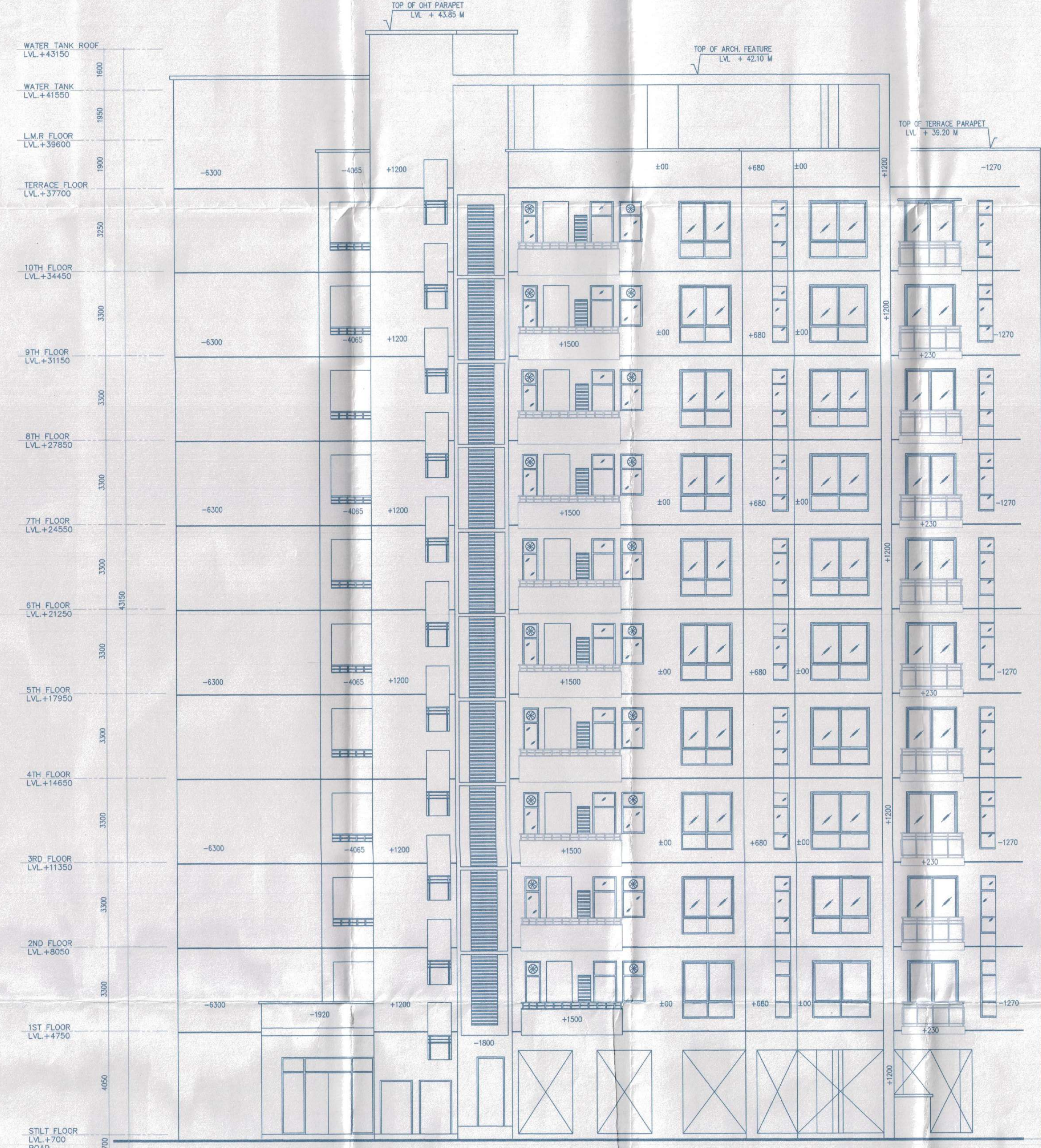
ELEVATION-03 BLOCK-K
