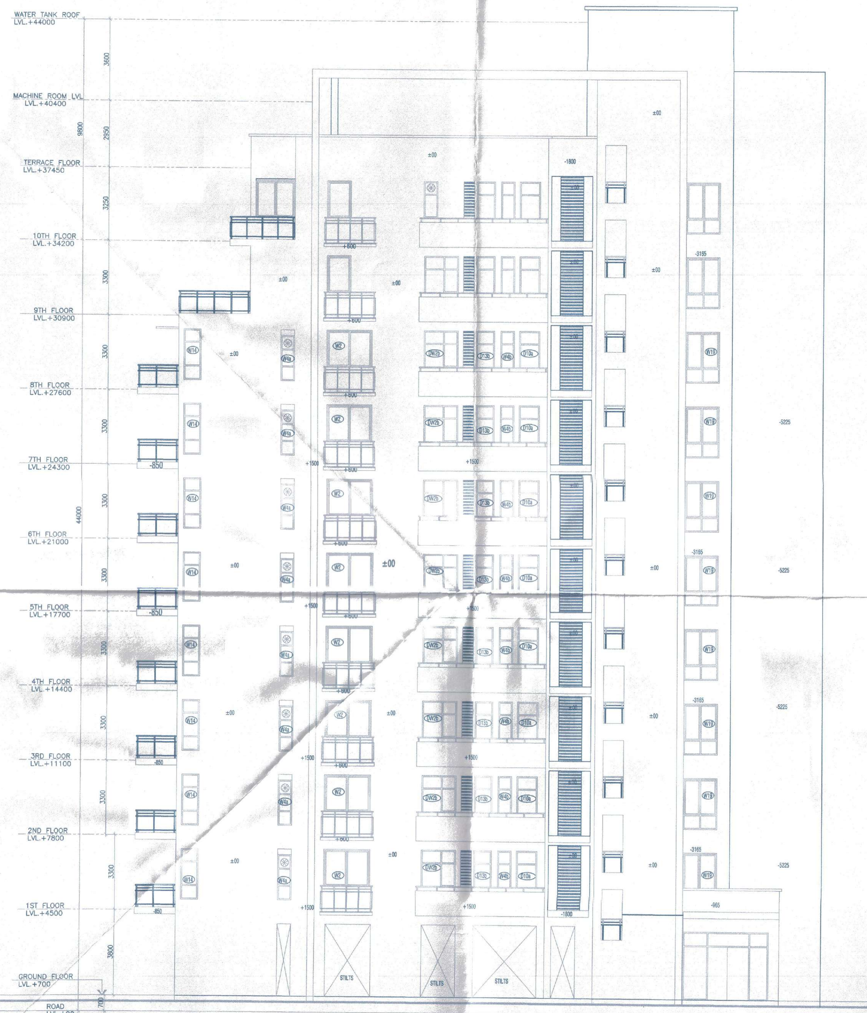
BLOCK-H ELEVATION-01
