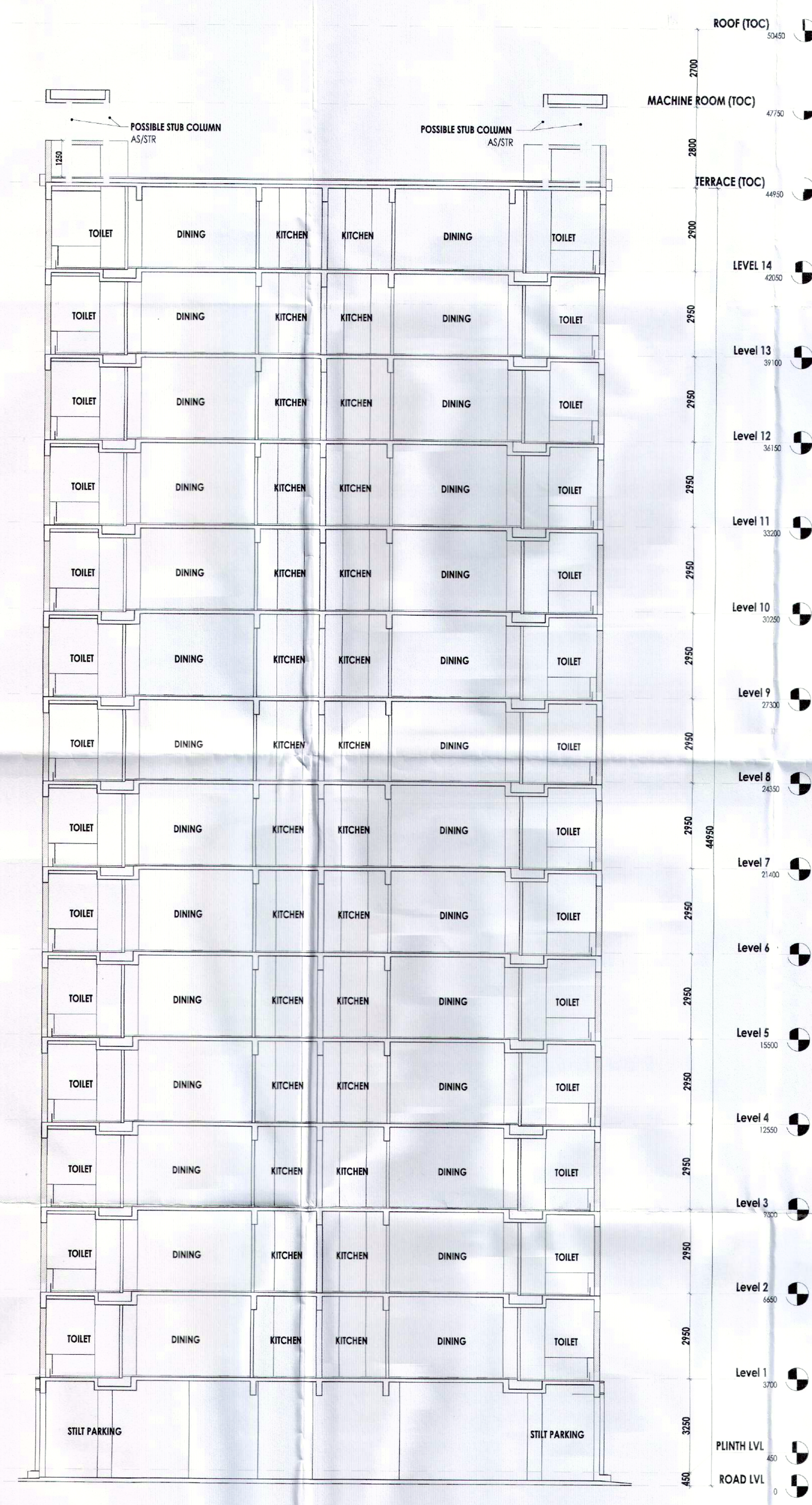
SECTION - 2
