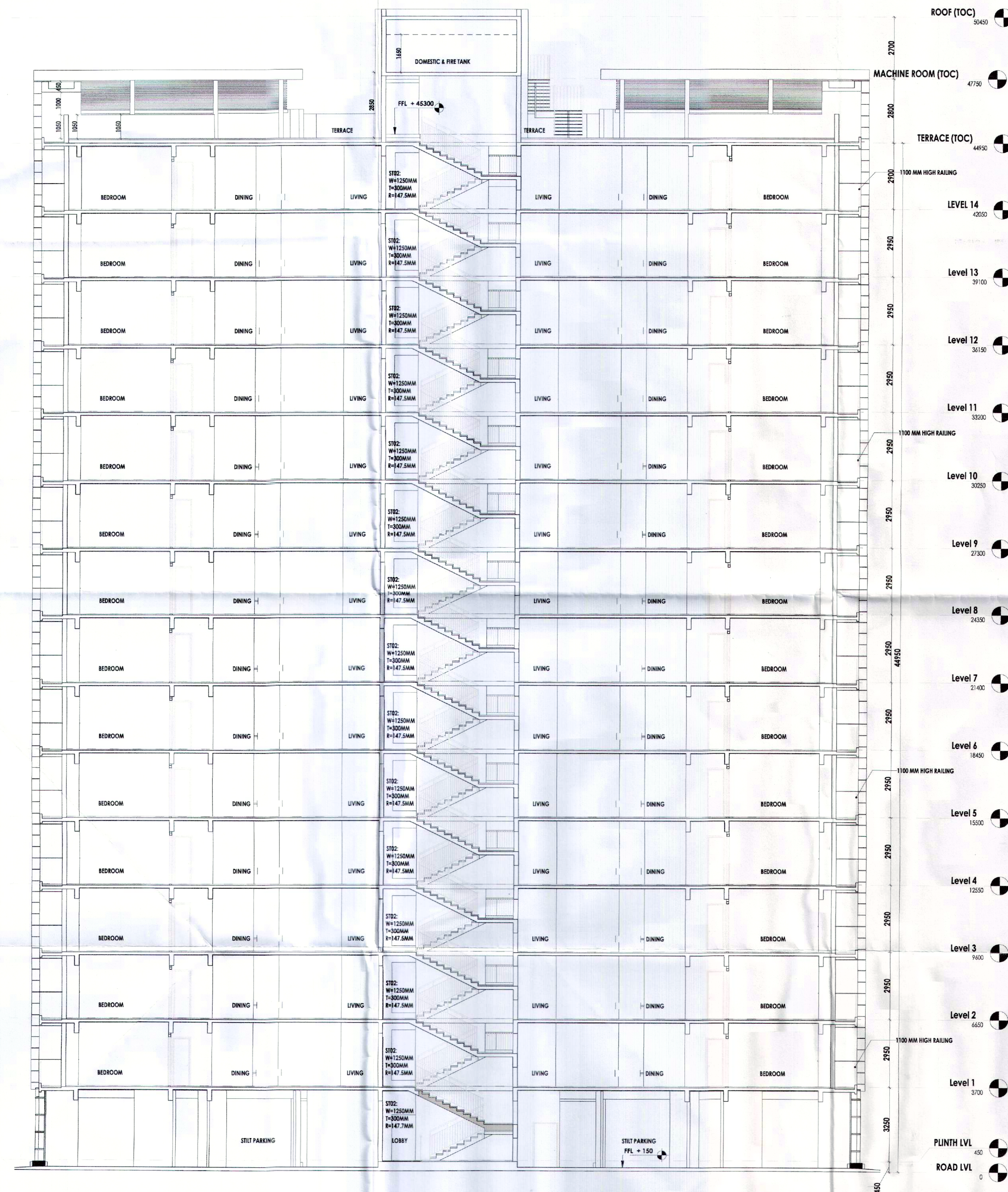
SECTION - 1
