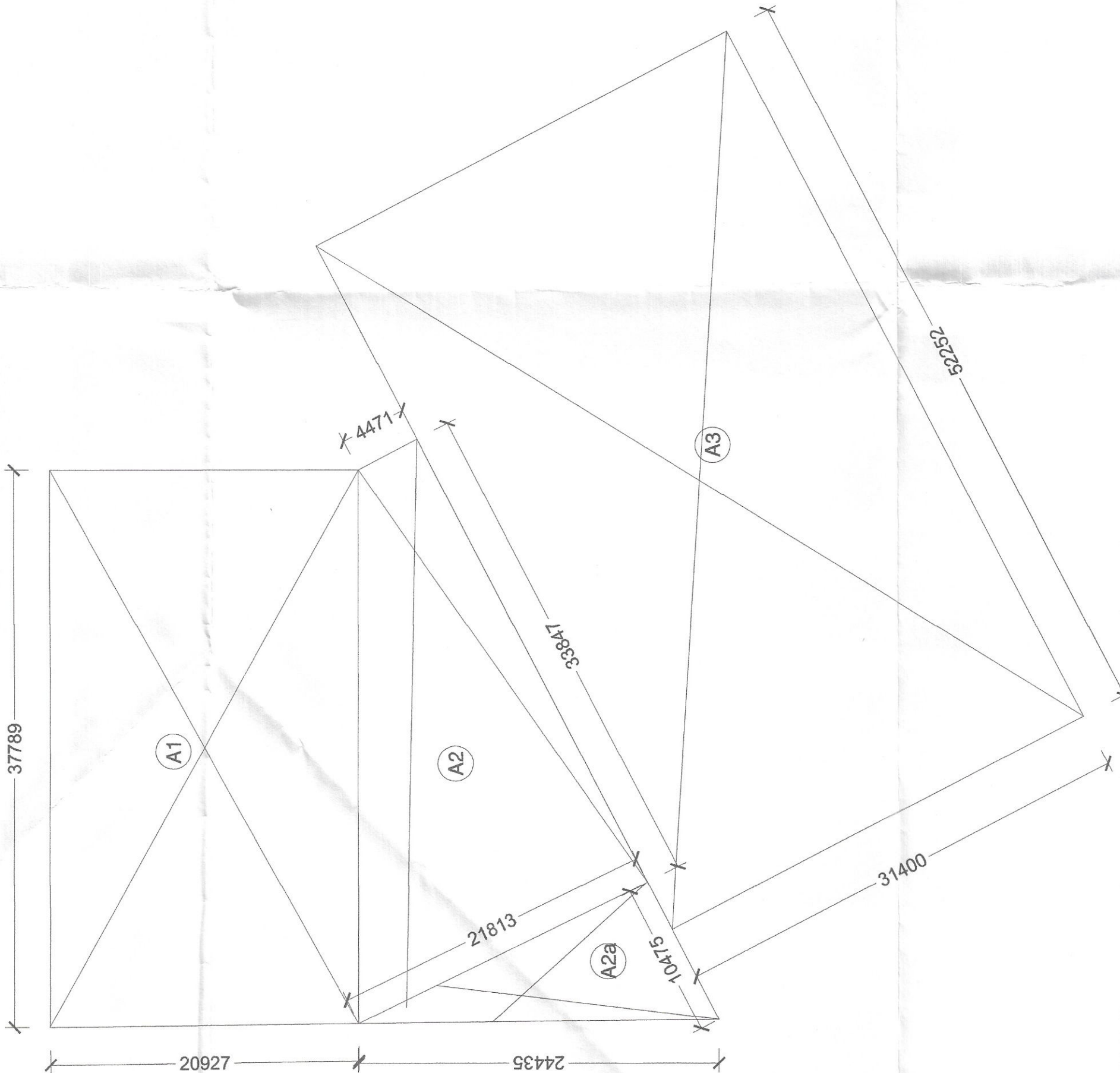
BASEMENT LEVEL -02 AREA PLAN (BLOCK A3)
