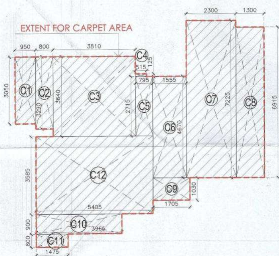
UNIT CARPET AREA DIAGRAM
