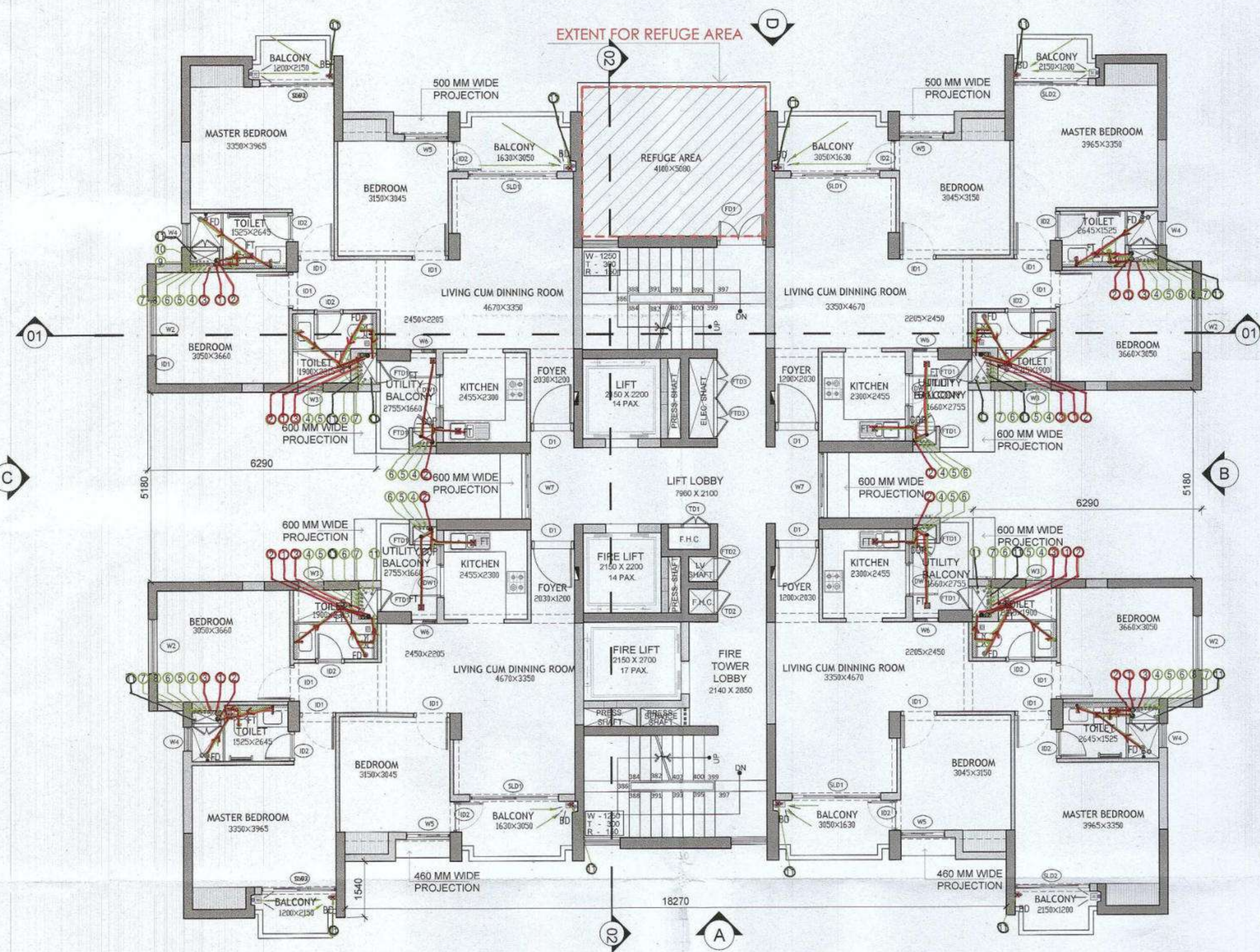
19th and 28th FLOOR PLAN
