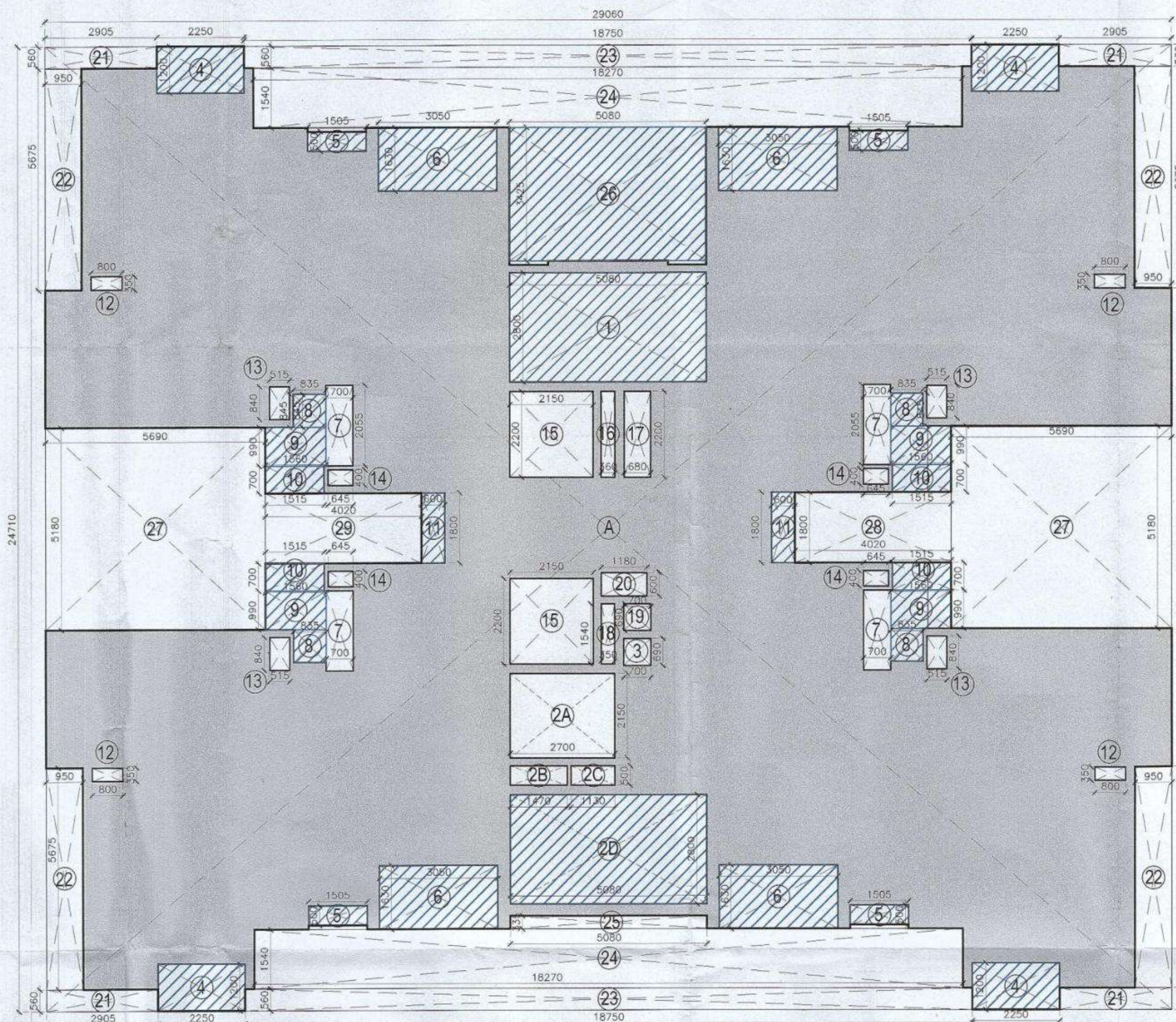
19th and 28th FLOOR AREA DIAGRAM
