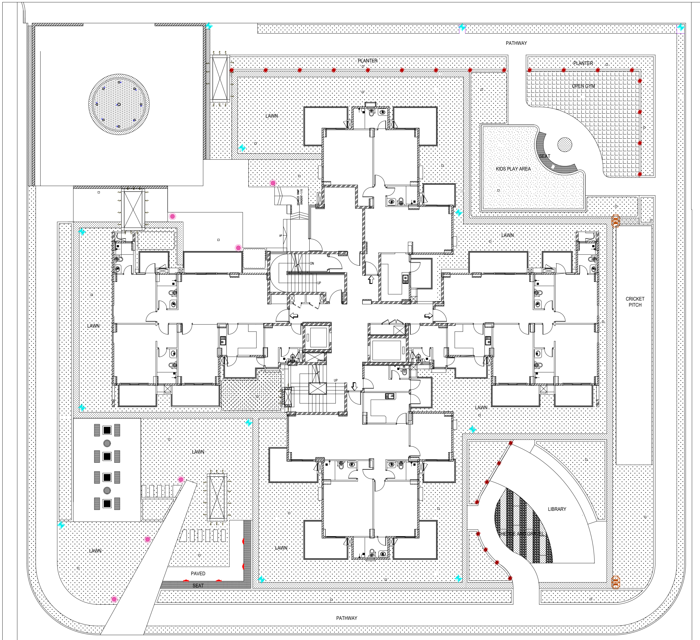
TOWER - G SCALE 1:150
