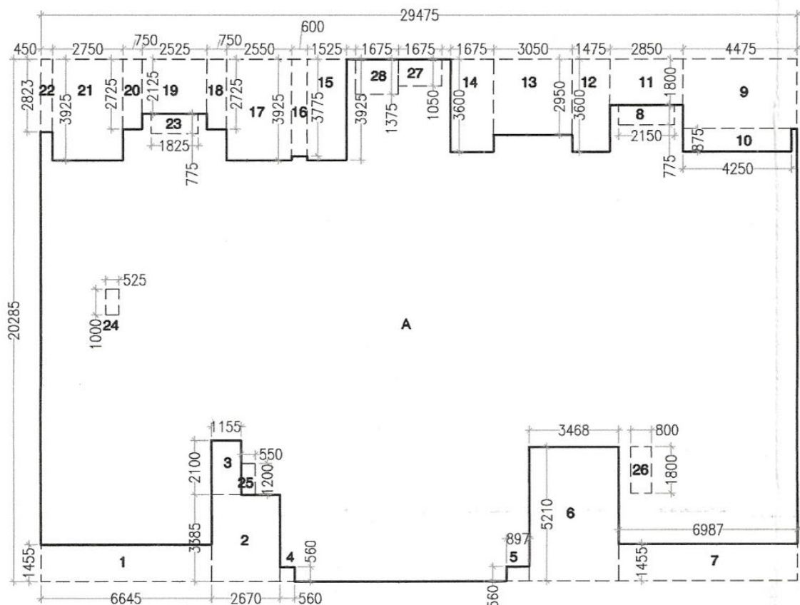
GROUND COVERAGE AREA DIAGRAM TOWER-2
