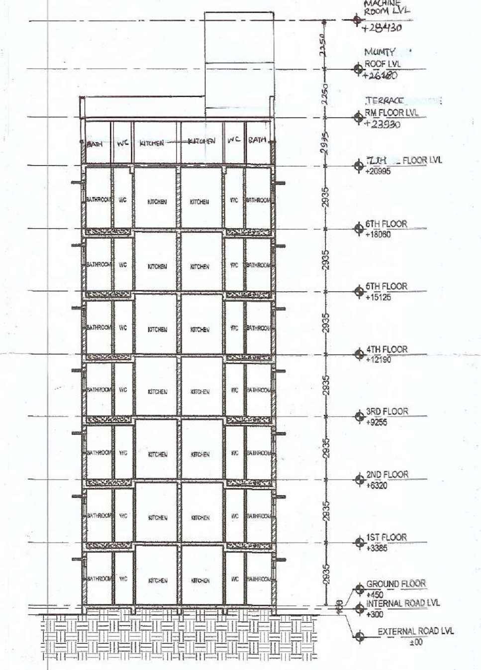
SECTION D1-D1' TOWER D
