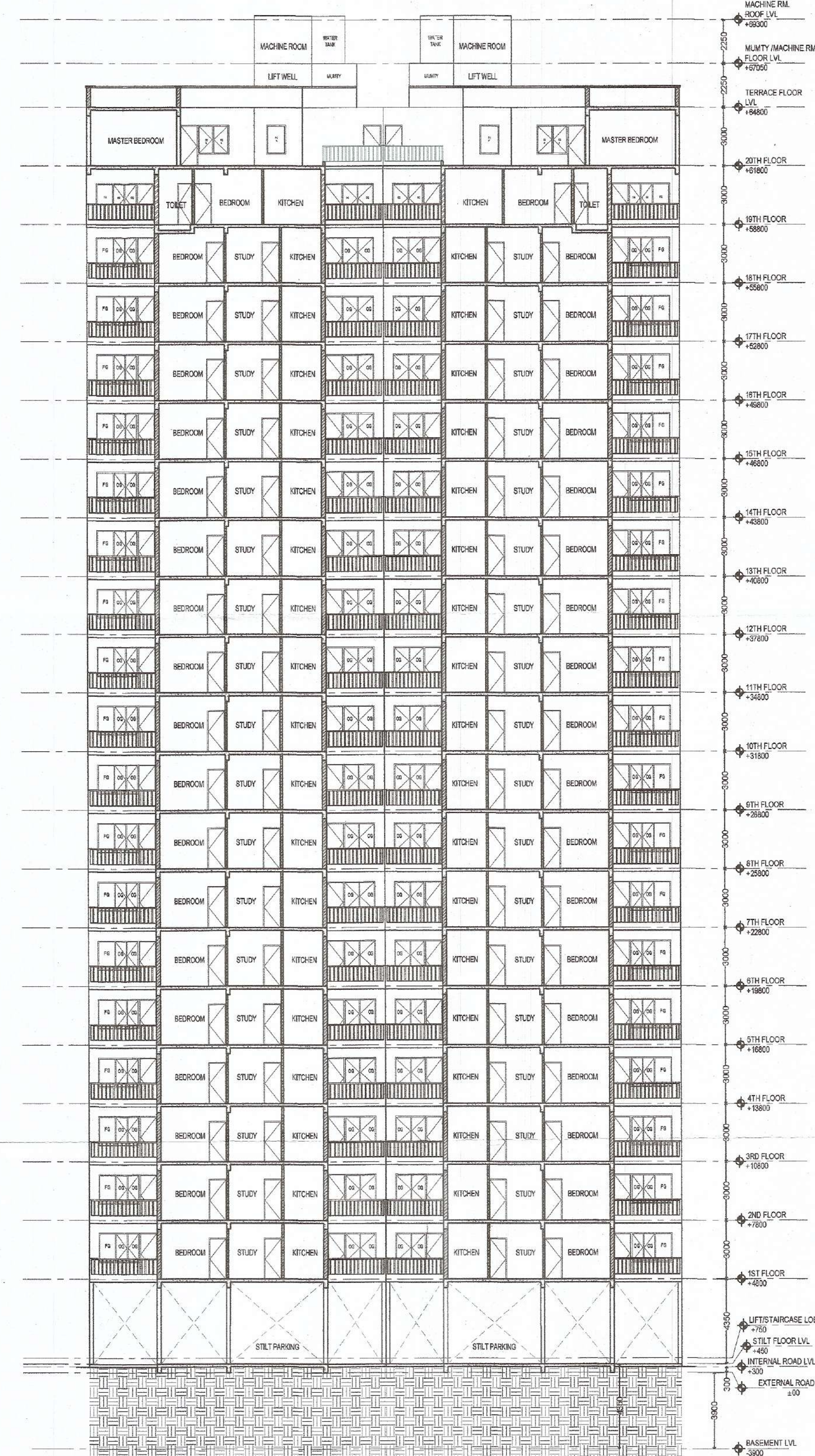
SECTION C1-C1' TOWER C
