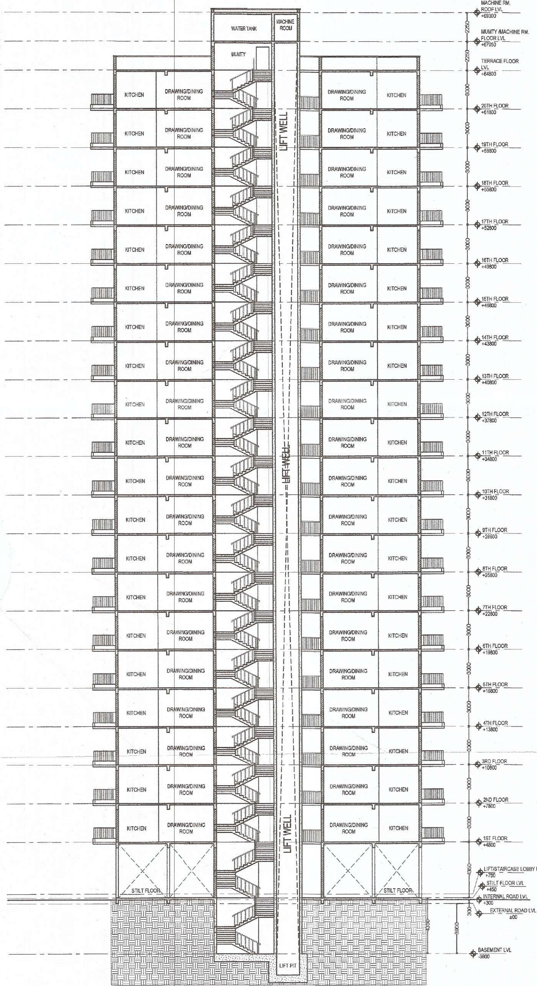
SECTION C-C' TOWER C
