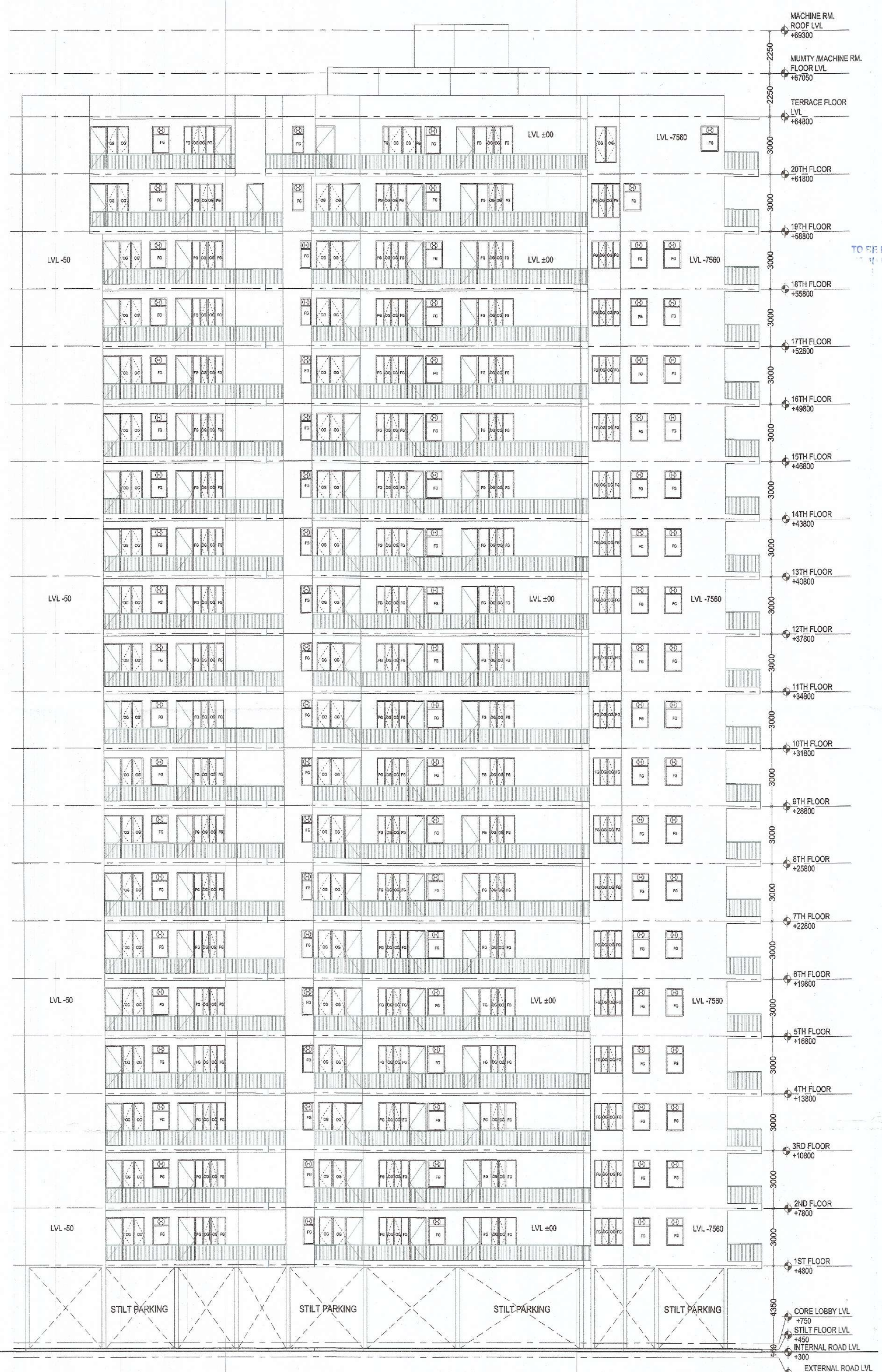
ELEVATION-4 TOWER B
