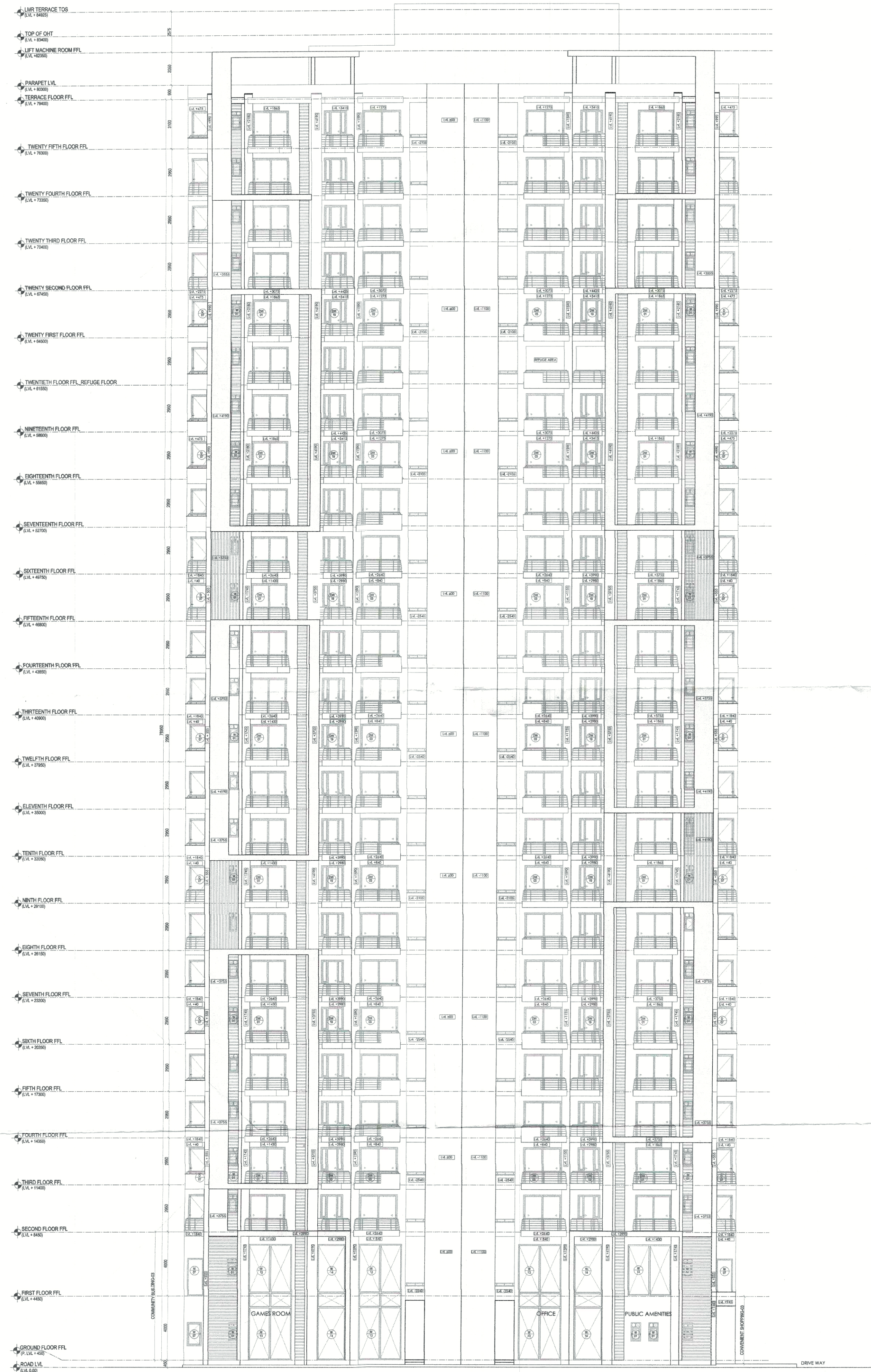
TOWER-04 ELEVATION 03
