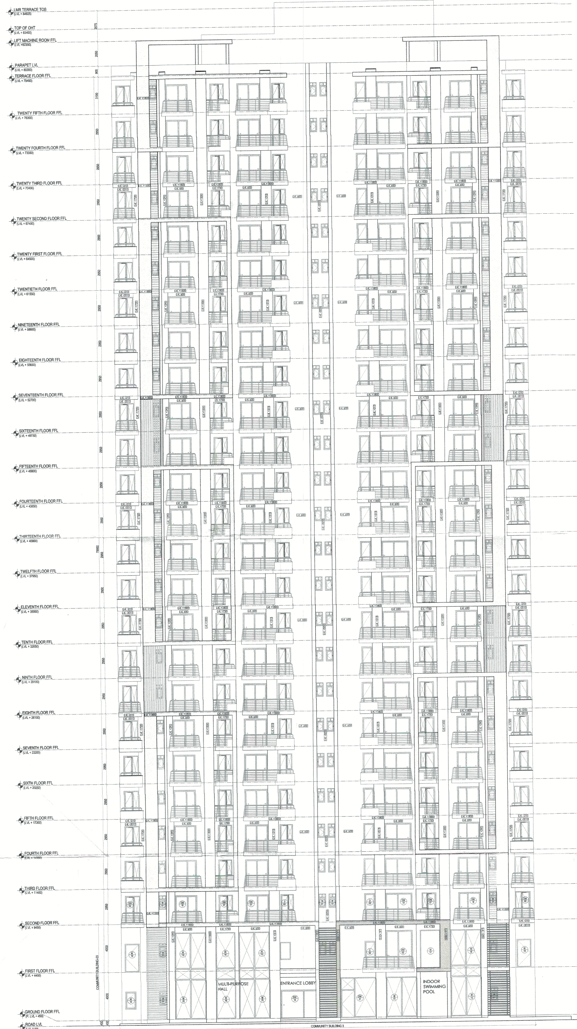
TOWER-04 ELEVATION 01
