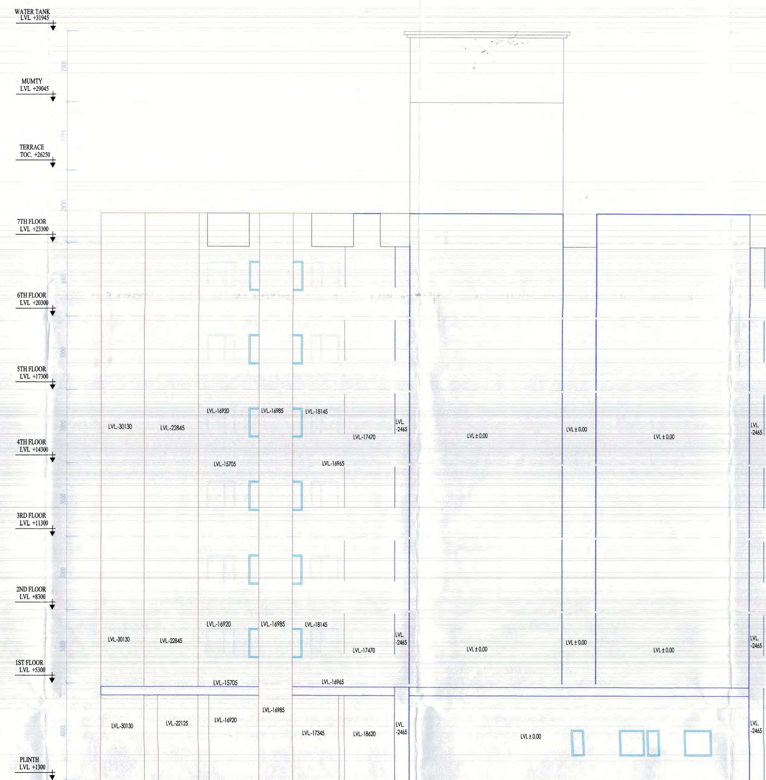
ELEVATION-B
