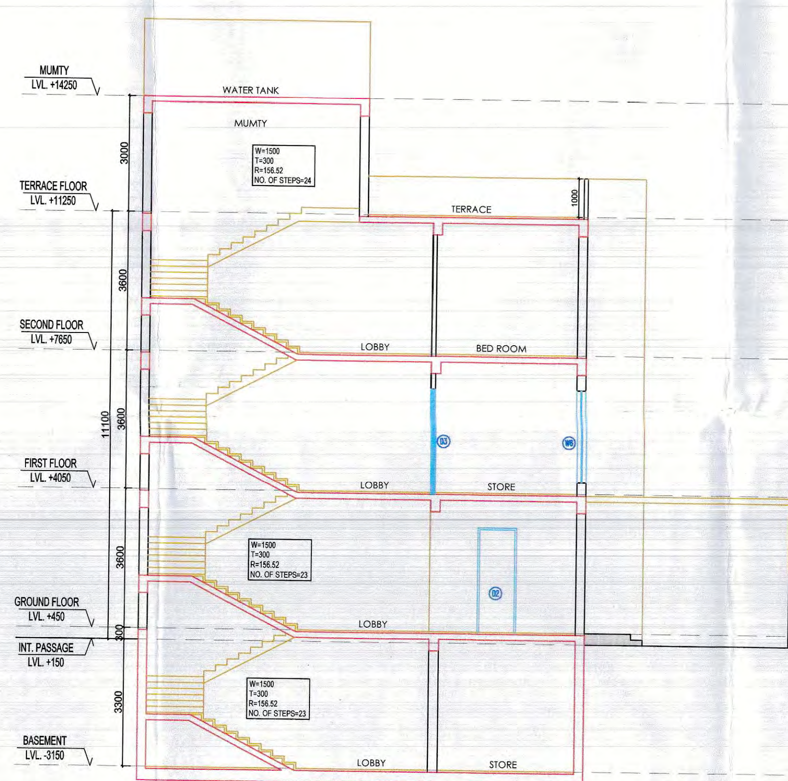
SECTION-1-1
