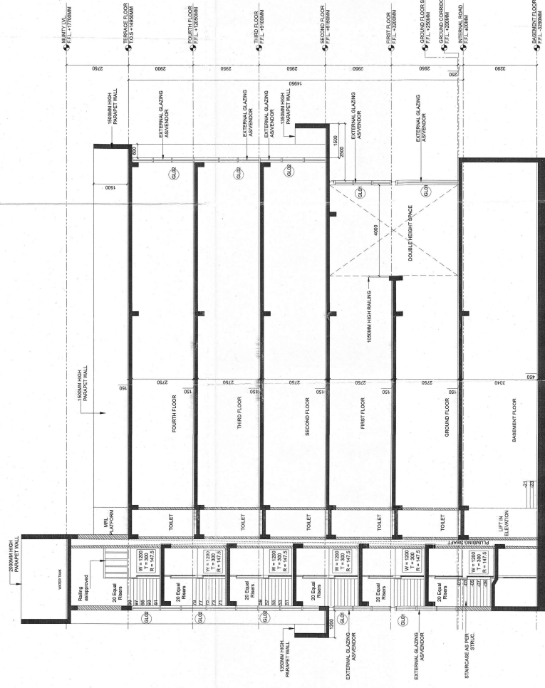
17 SECTION A
