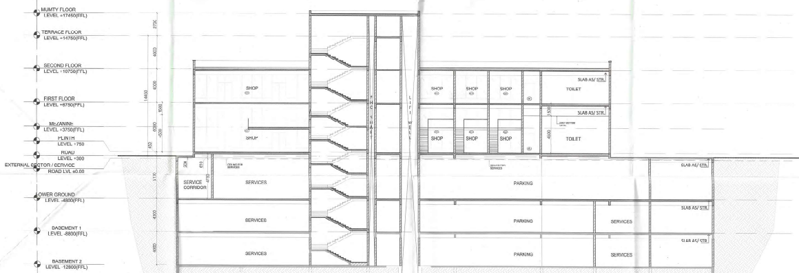
SECTION 2 SCALE 1:150
