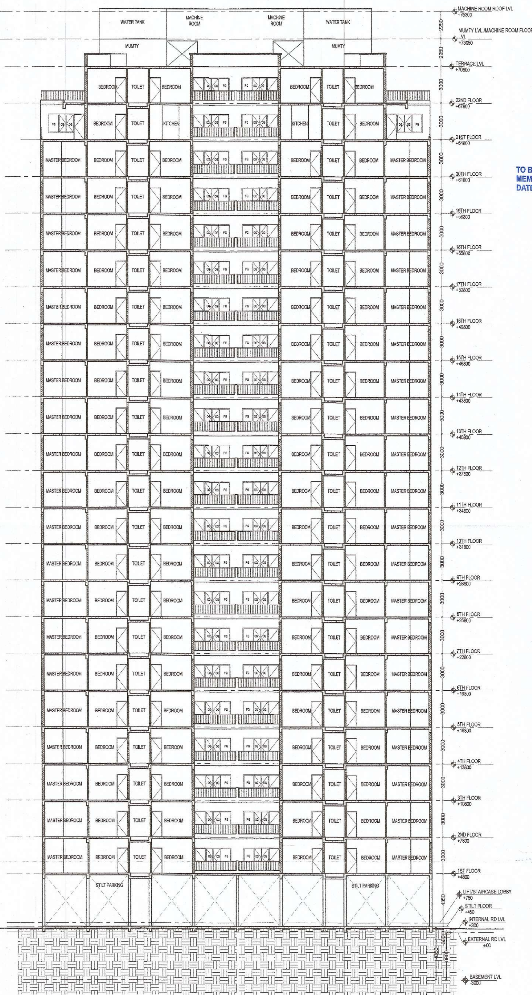
SECTION A1-A1' TOWER A
