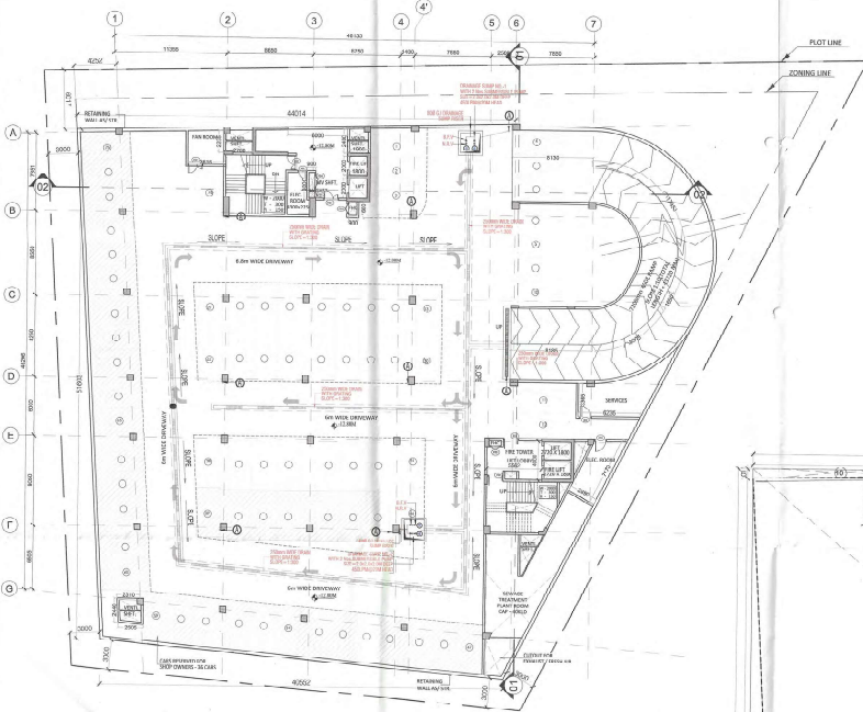
BASEMENT 3 PLAN SCALE 1:200
