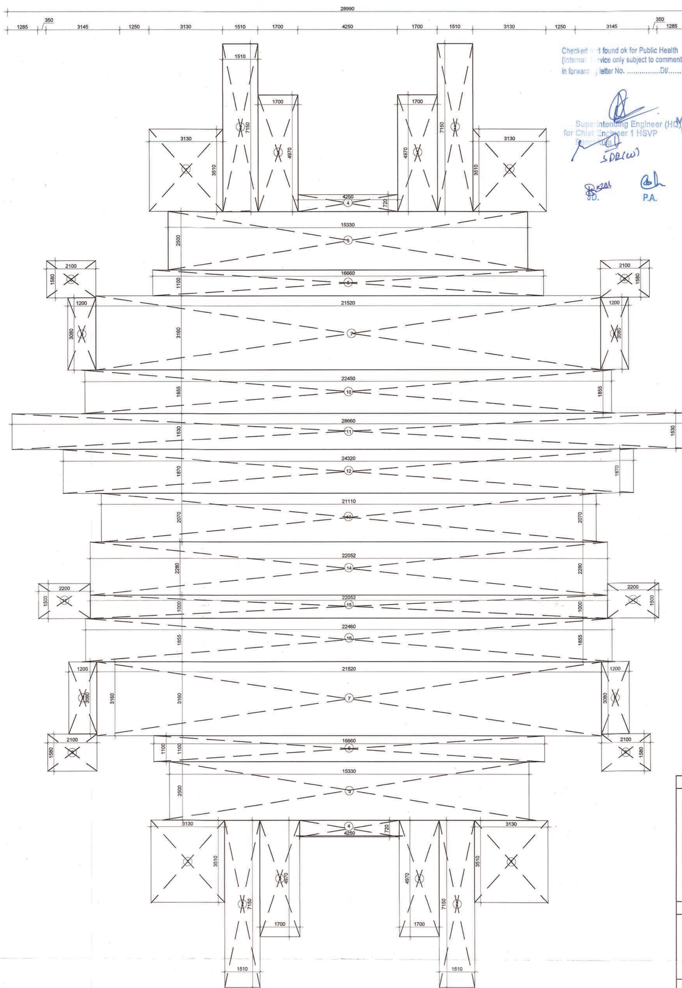
2 1ST -20TH FLOOR AREA DETAIL - TOWER 04
