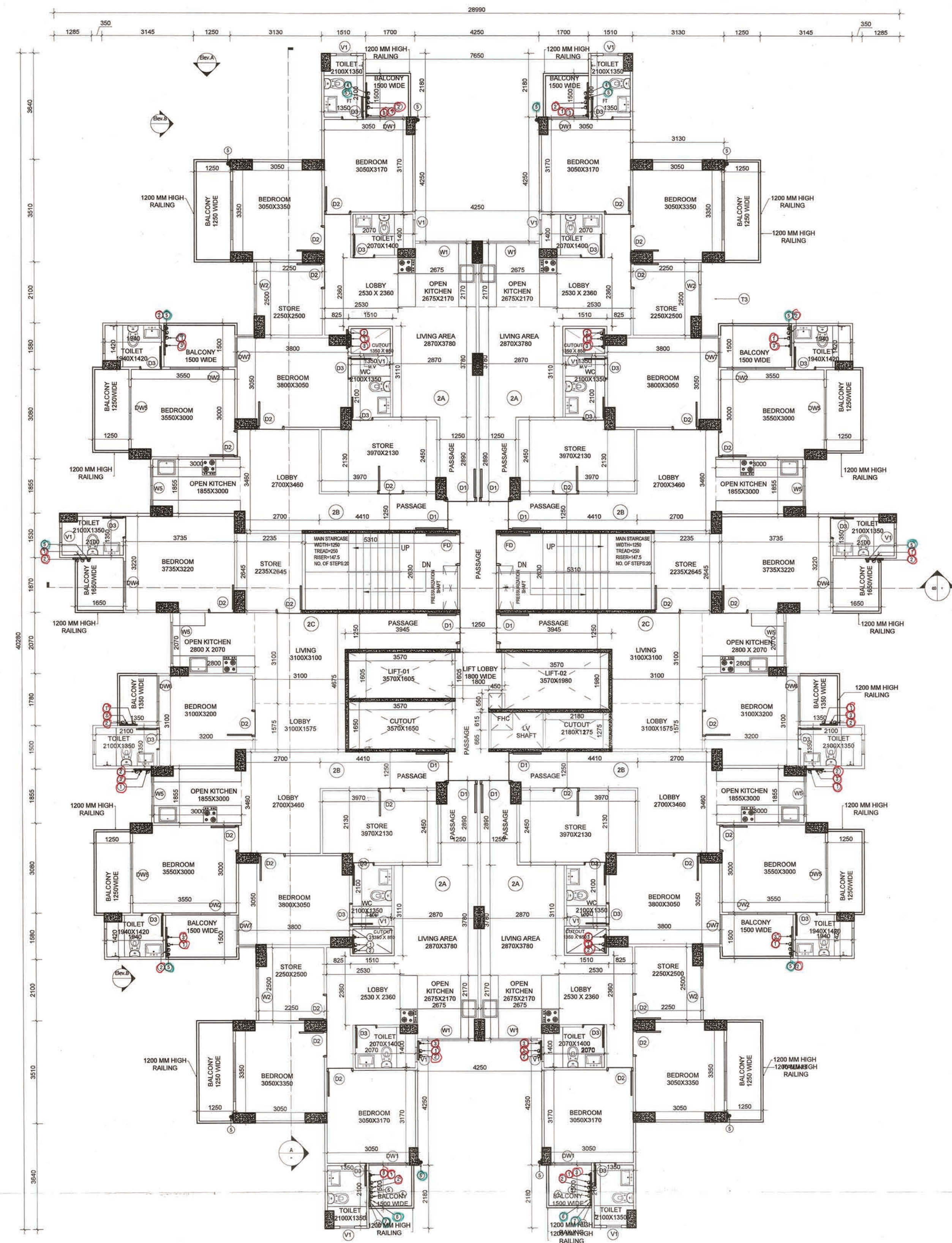
TYPICAL FLOOR AREA DETAIL (1st to 20th Floor)
