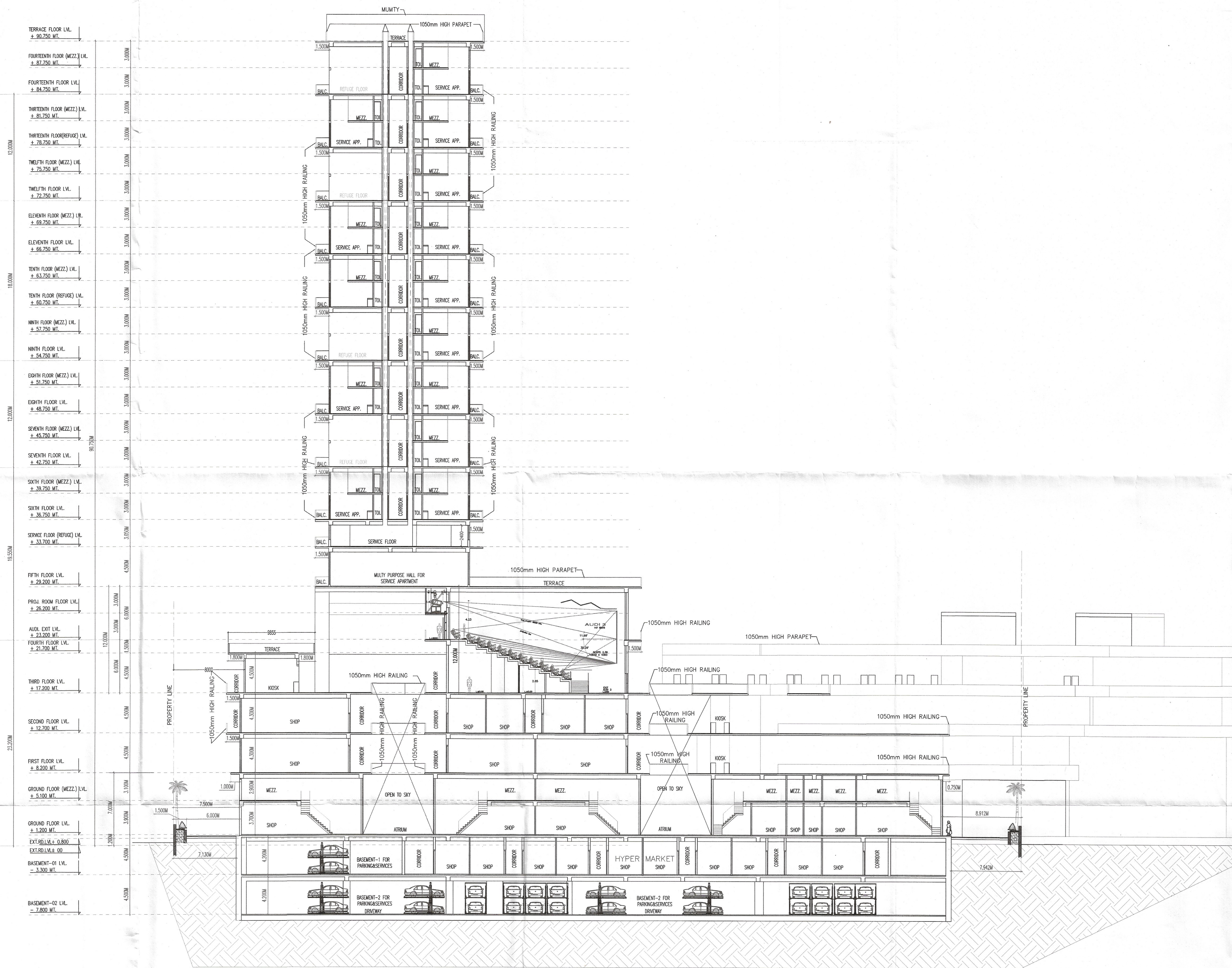
SECTION -AA
