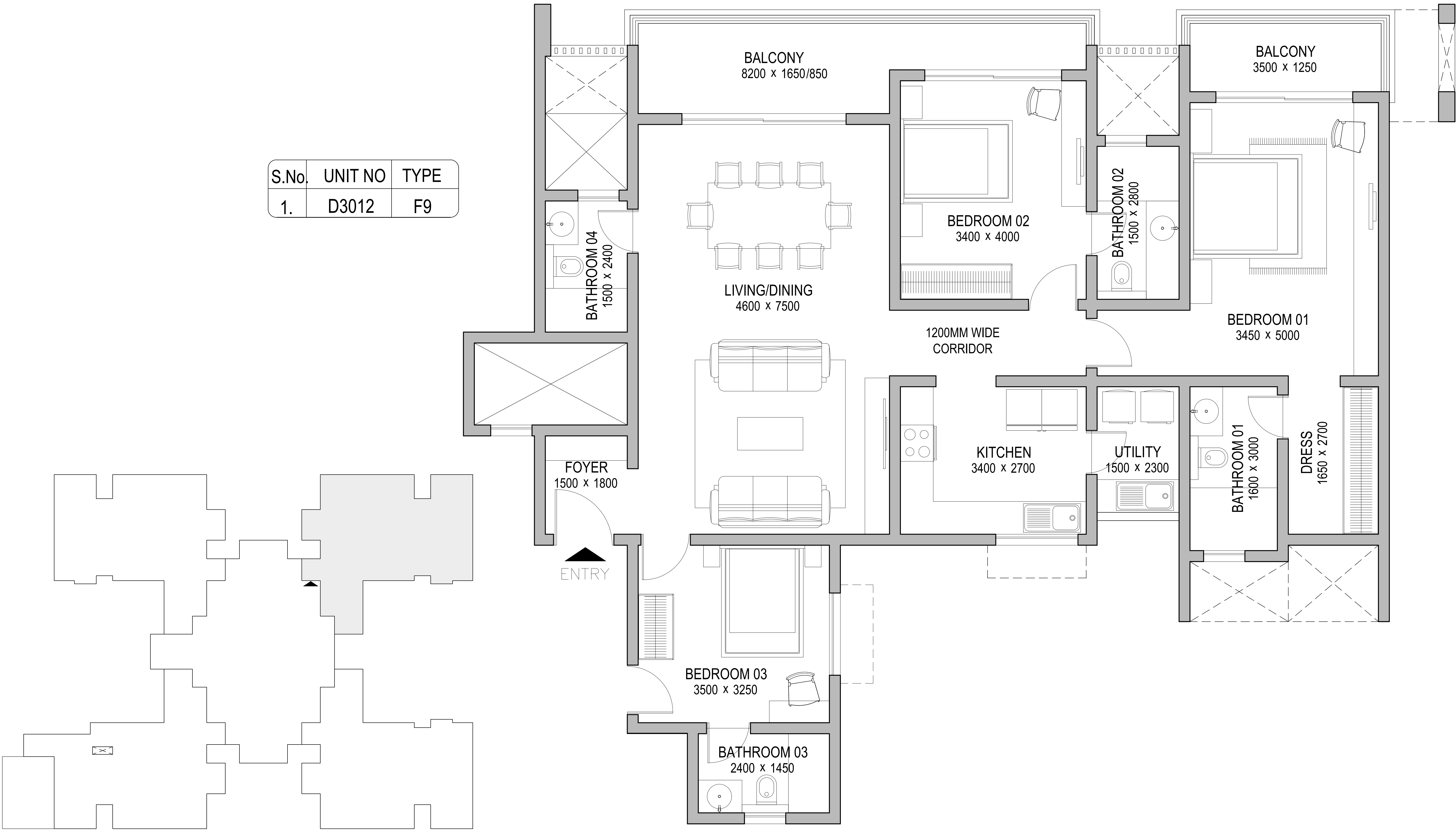
01 UNIT PLAN SCALE 1:100
