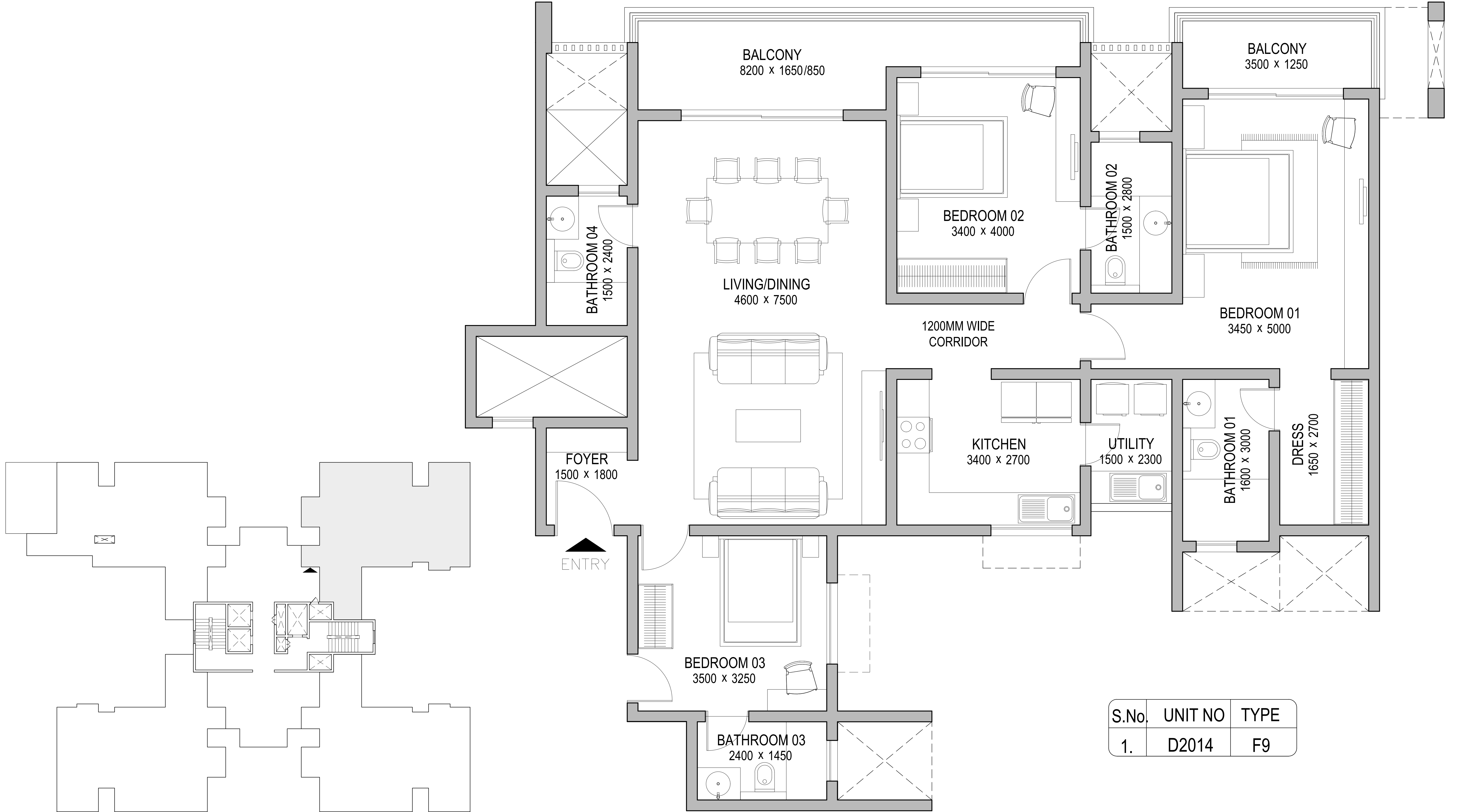
01 UNIT PLAN SCALE 1:100
