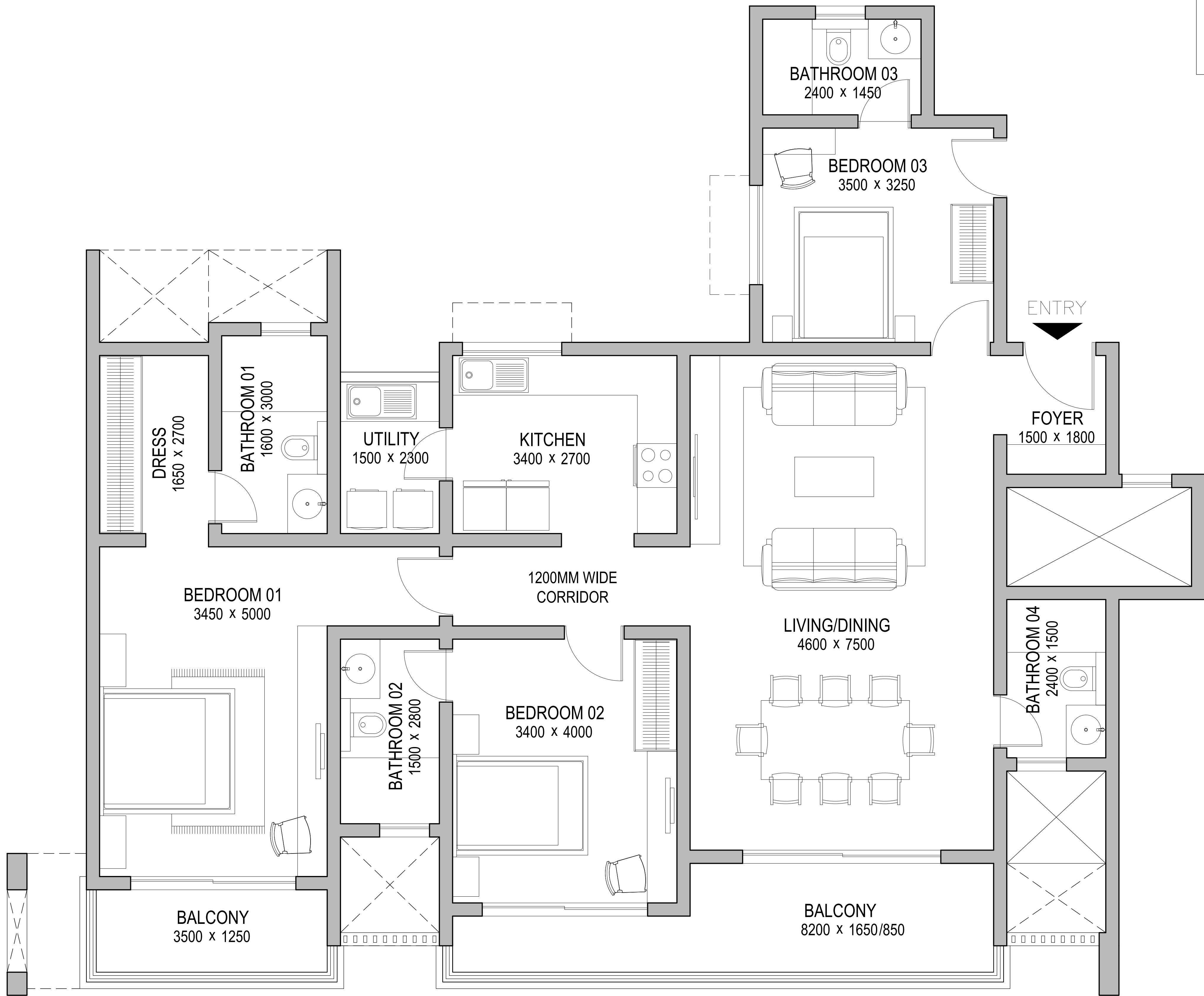
01 UNIT PLAN SCALE 1:100
