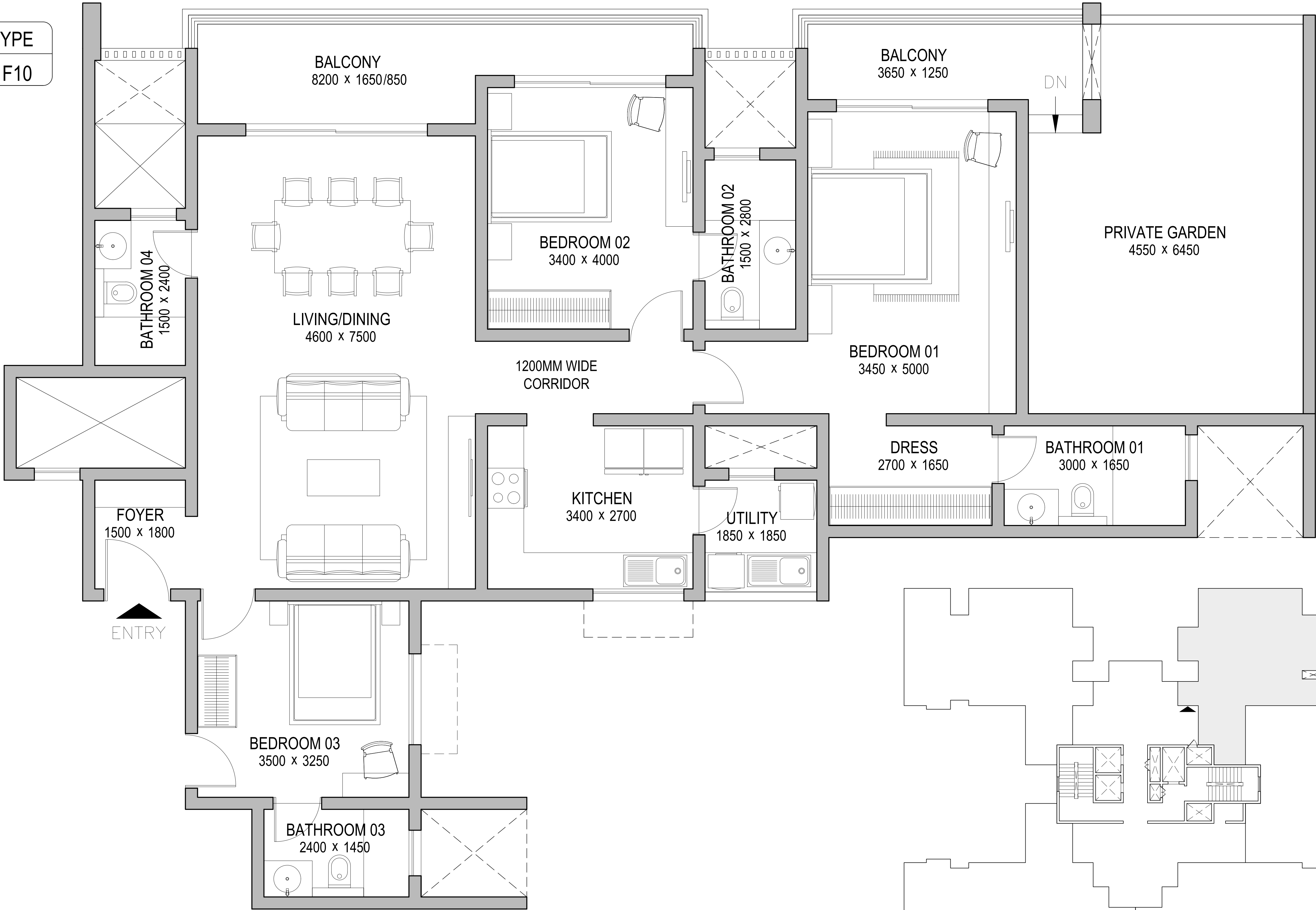
01 UNIT PLAN SCALE 1:100
