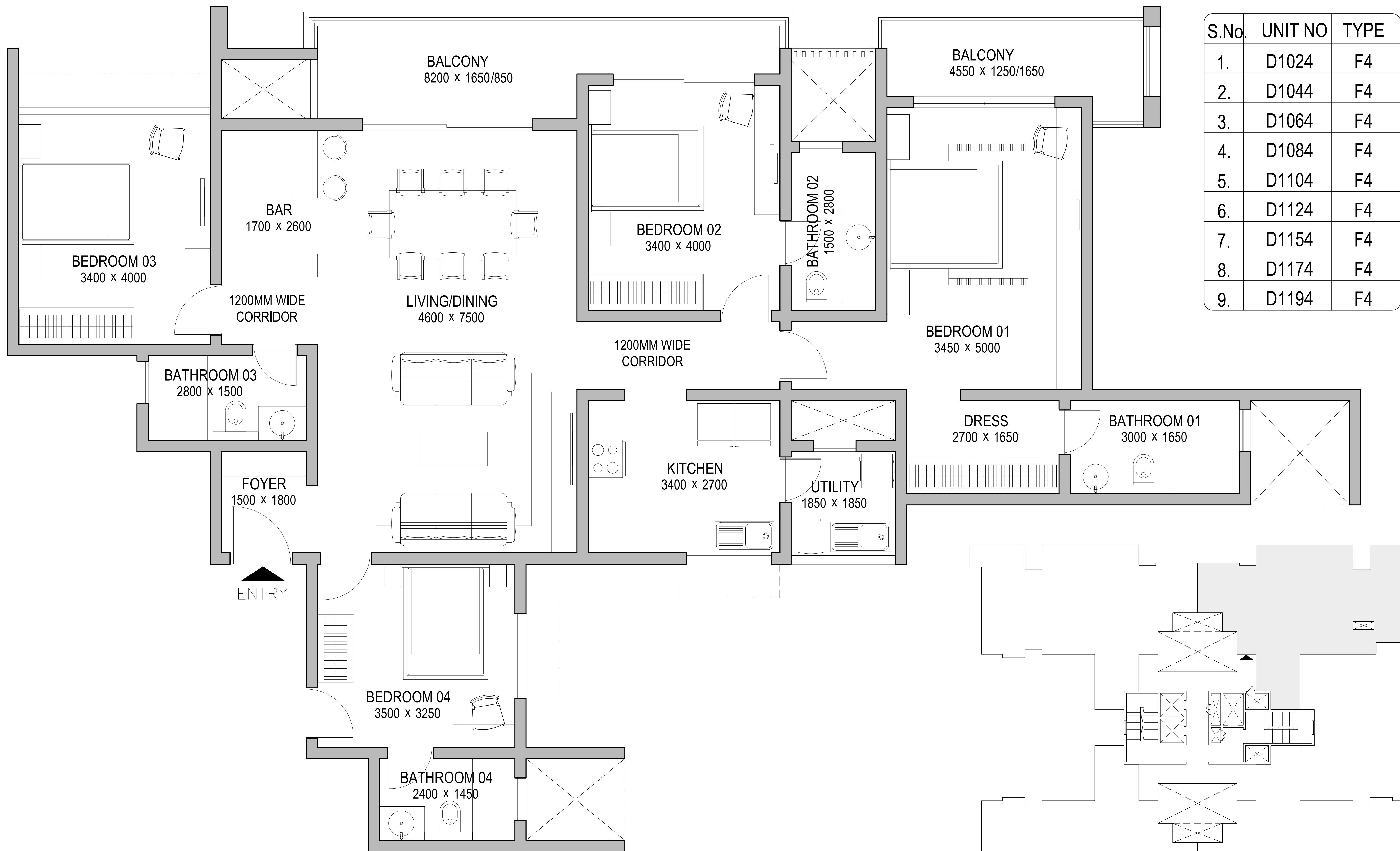
01 UNIT PLAN SCALE 1:100
