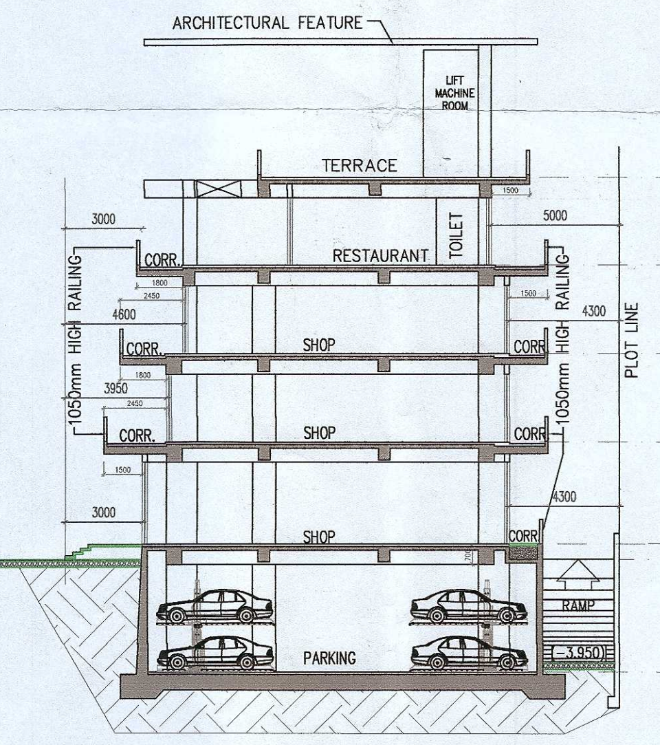
SECTION AT:- B1-B1
