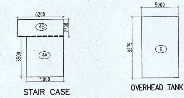
AREA DIAGRAM-TERRACE FLOOR
