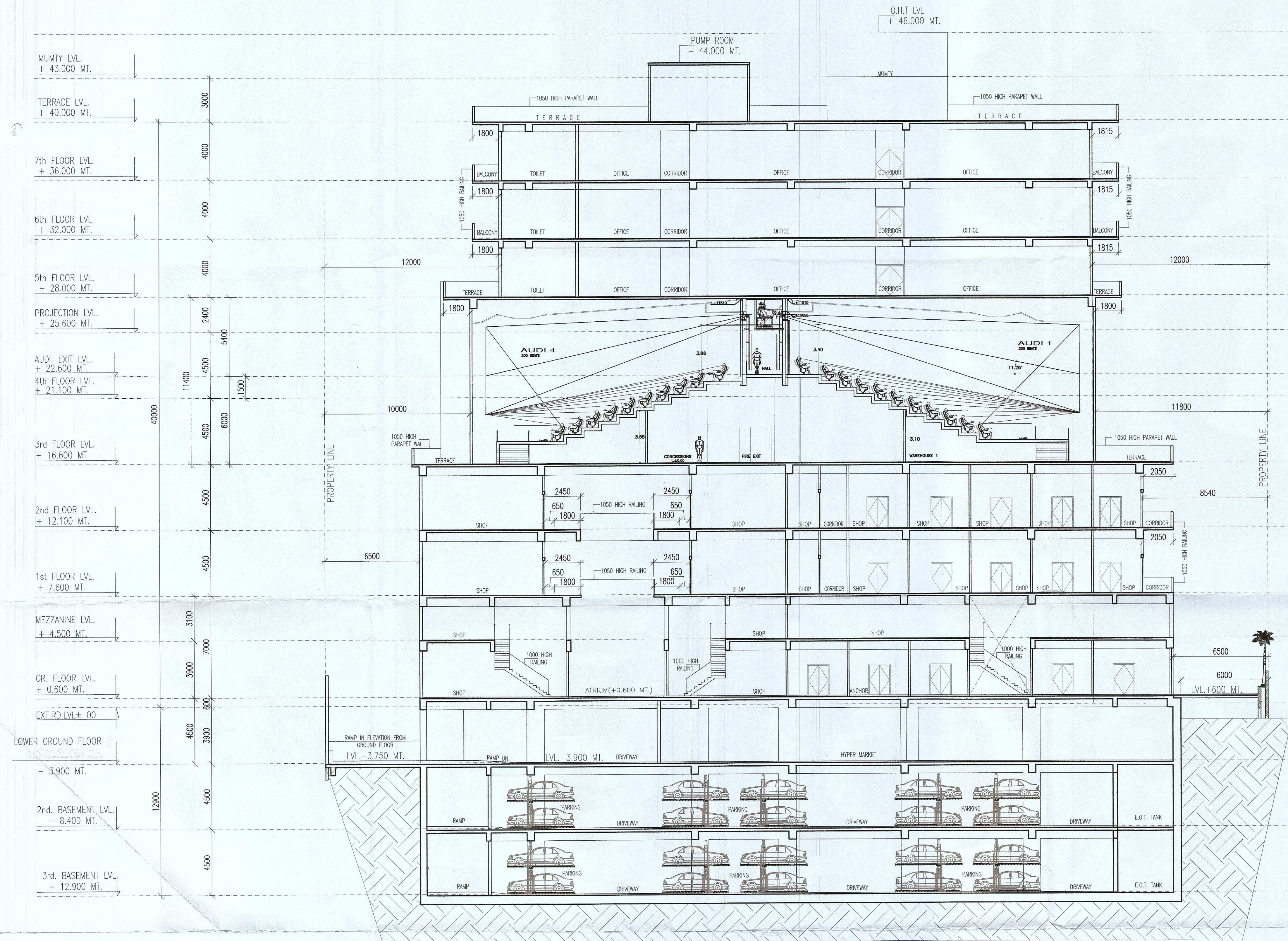
SECTION - B-B
