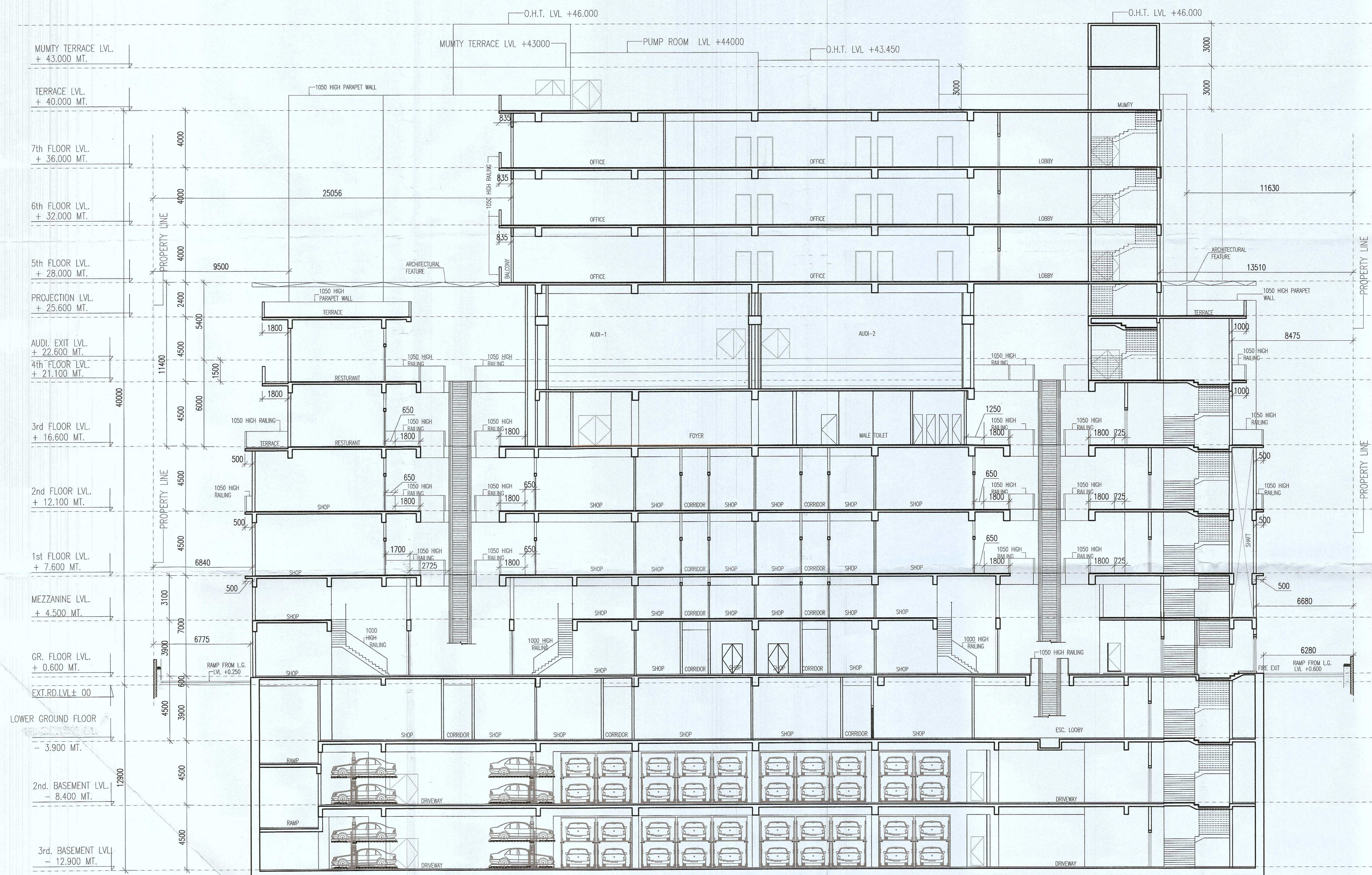
SECTION -A-A
