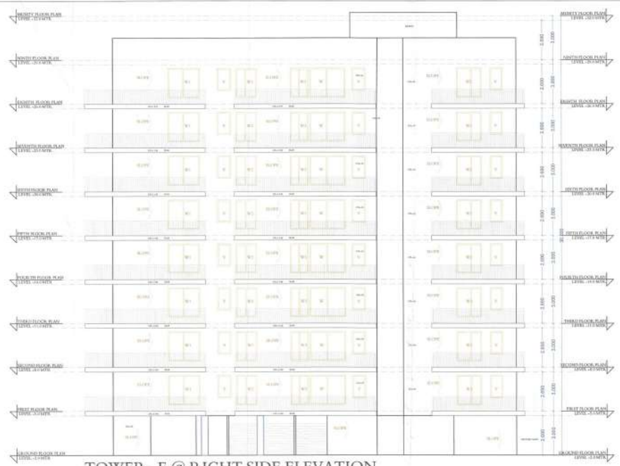
TOWER -E @ RIGHT SIDE ELEVATION
