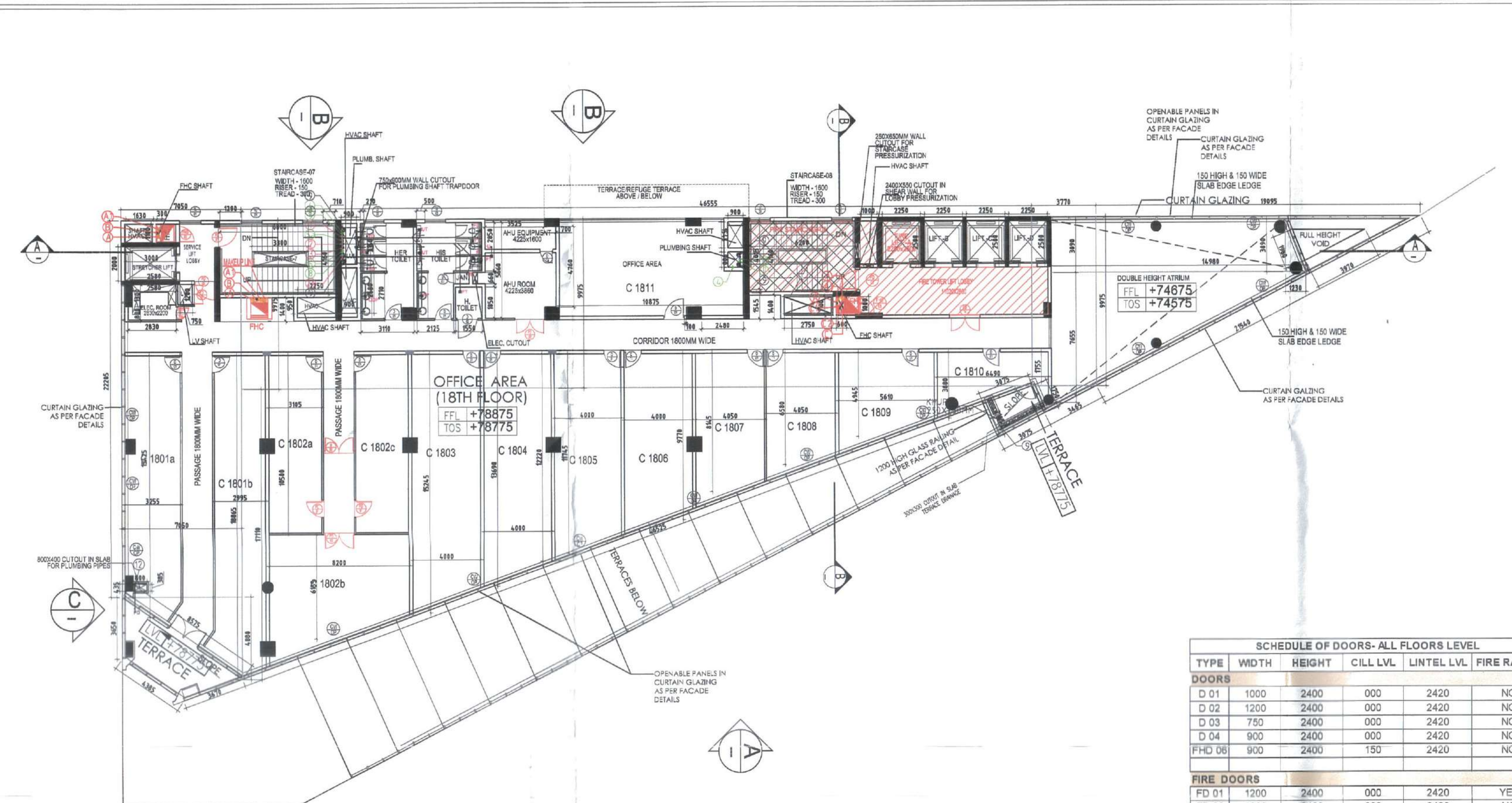
EIGHTEENTH FLOOR PLAN (LVL+78875MM) SCALE 1 : 125
