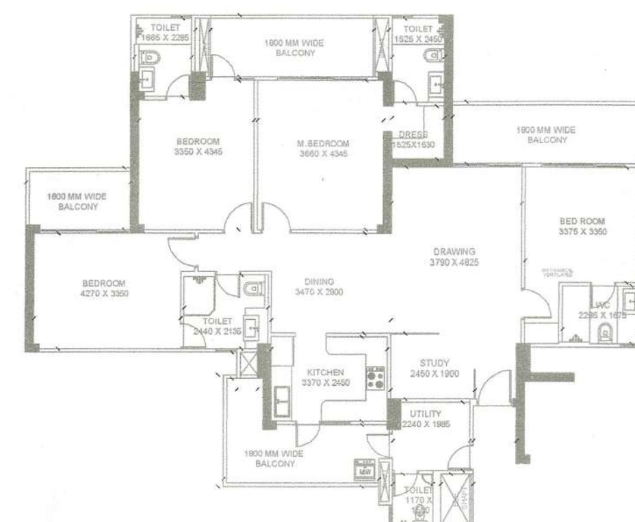
4BHK (INCLUDING 1SPR) +STUDY+UTILITY (TOWER- 5A) CARPET AREA
