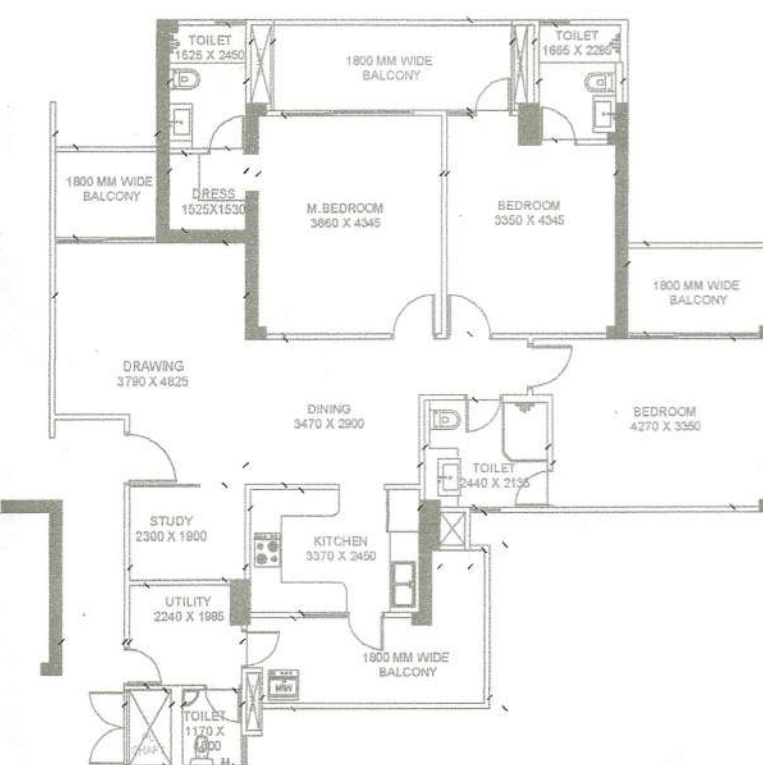
3BHK+STUDY+UTILITY (TOWER- 5A) CARPET AREA
