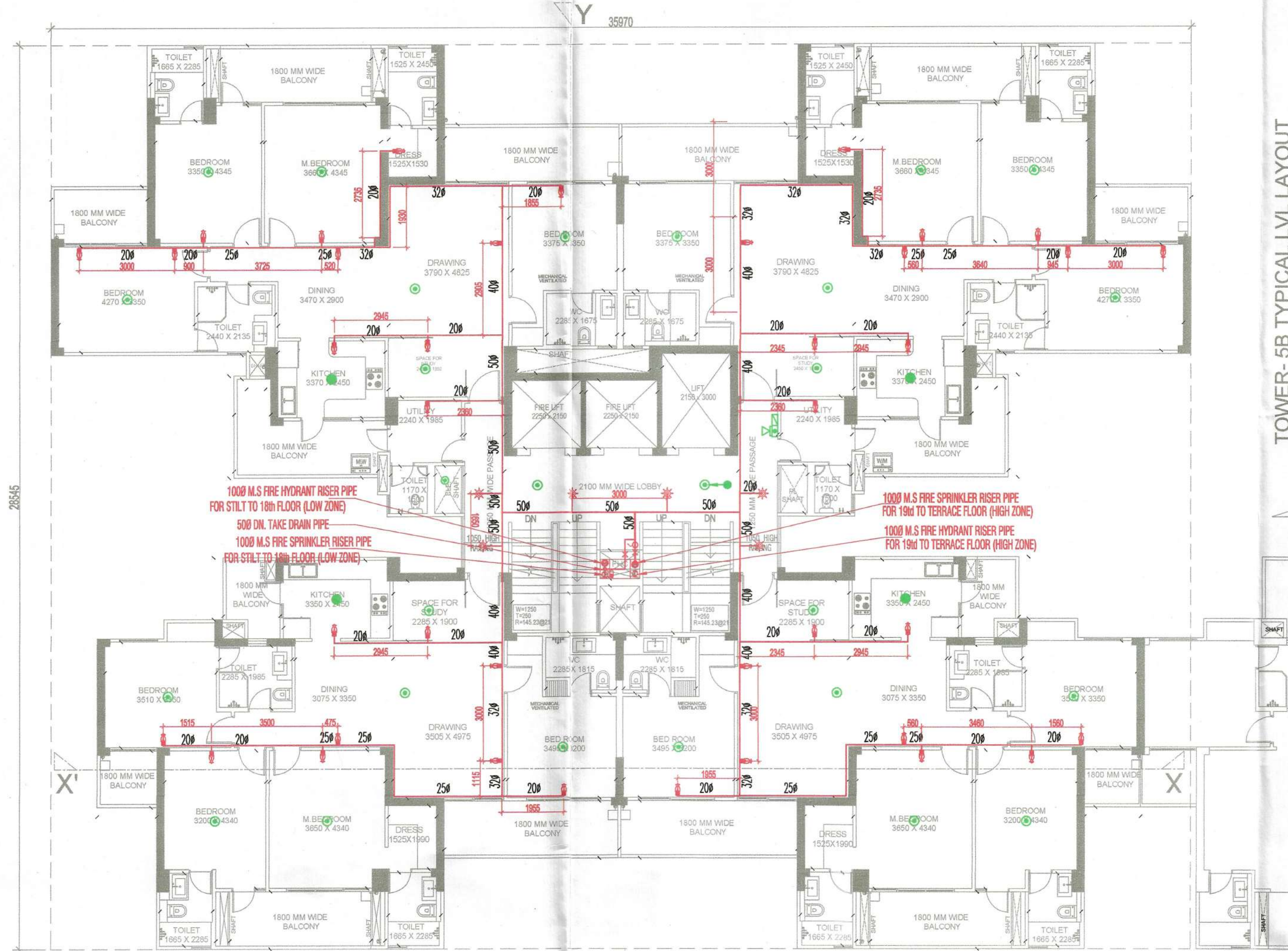
TOWER- 5A TYPICAL LVL LAYOUT (LEVEL - 6th to 19th, 21st to 29th & 31st to 36th)
