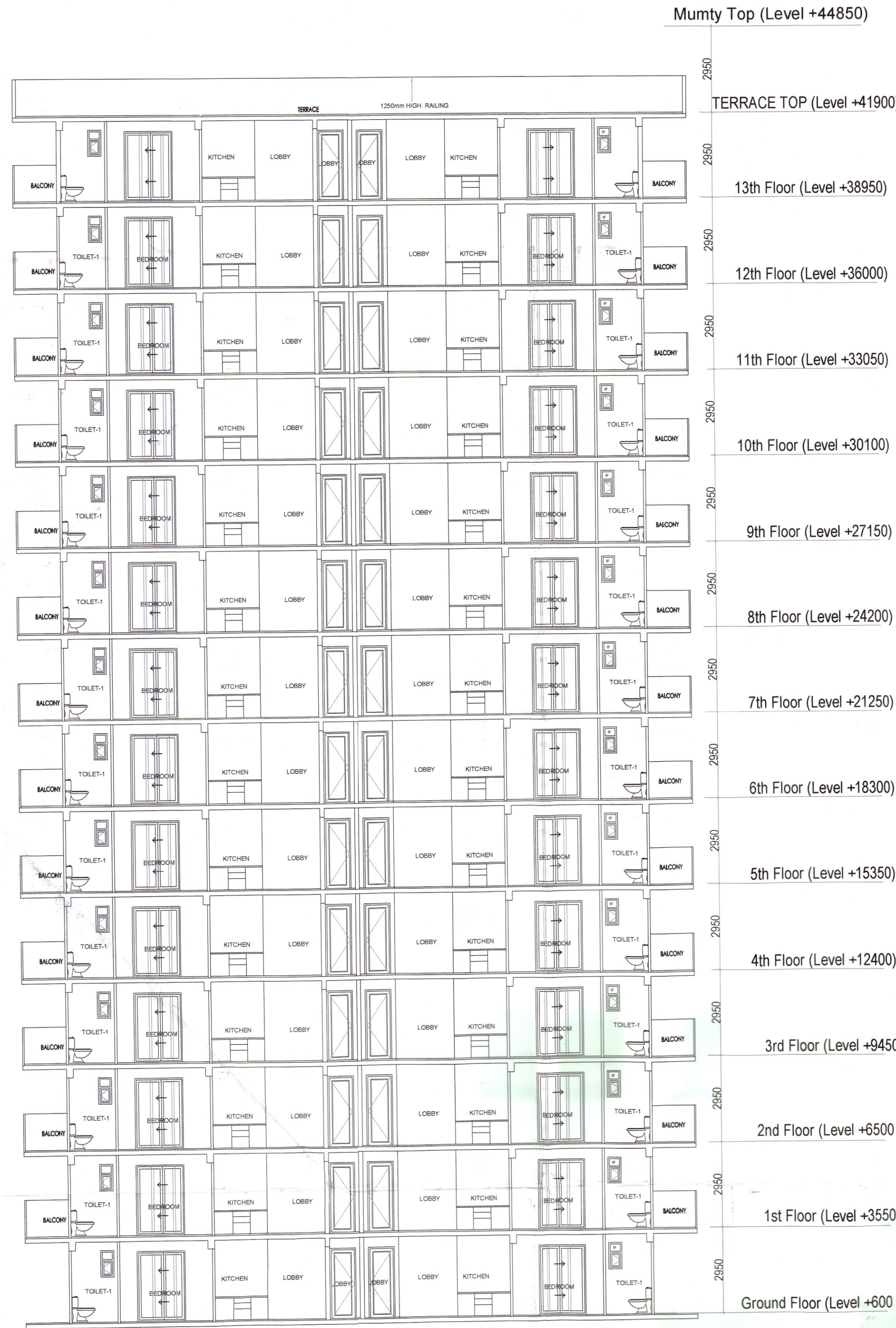
SECTION AT B-b
