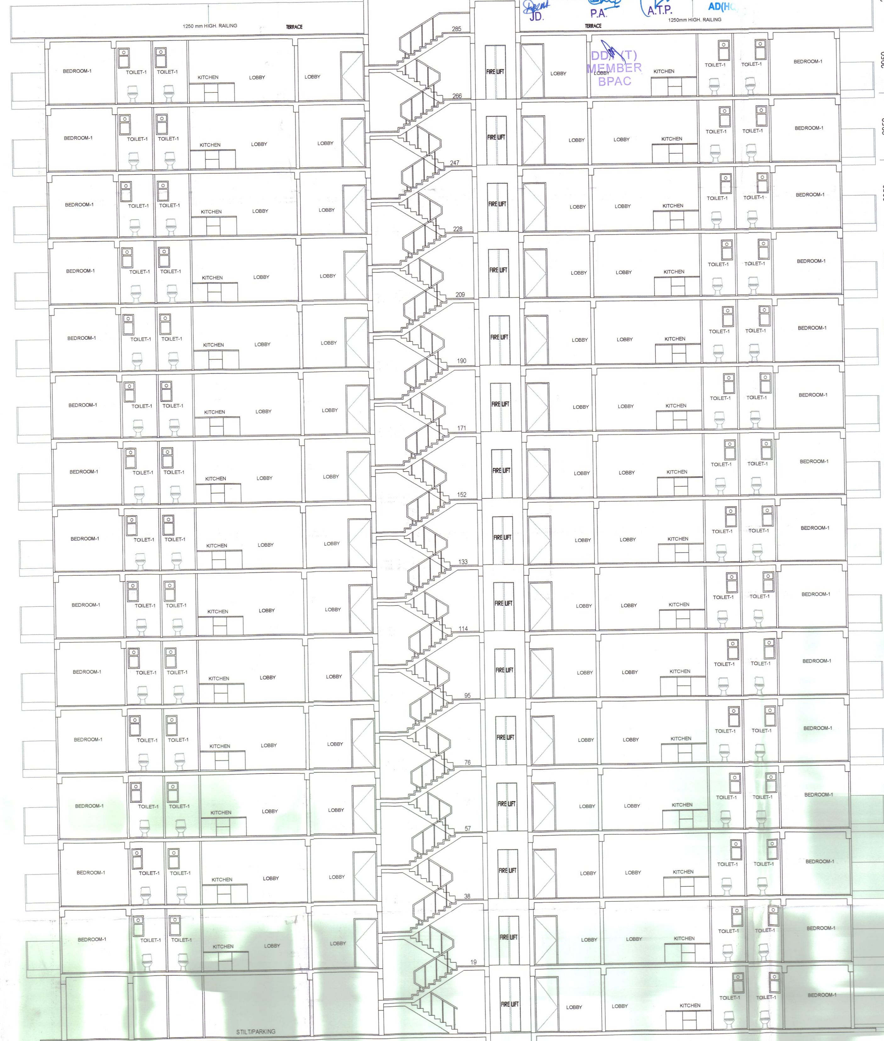
SECTION AT A-a
