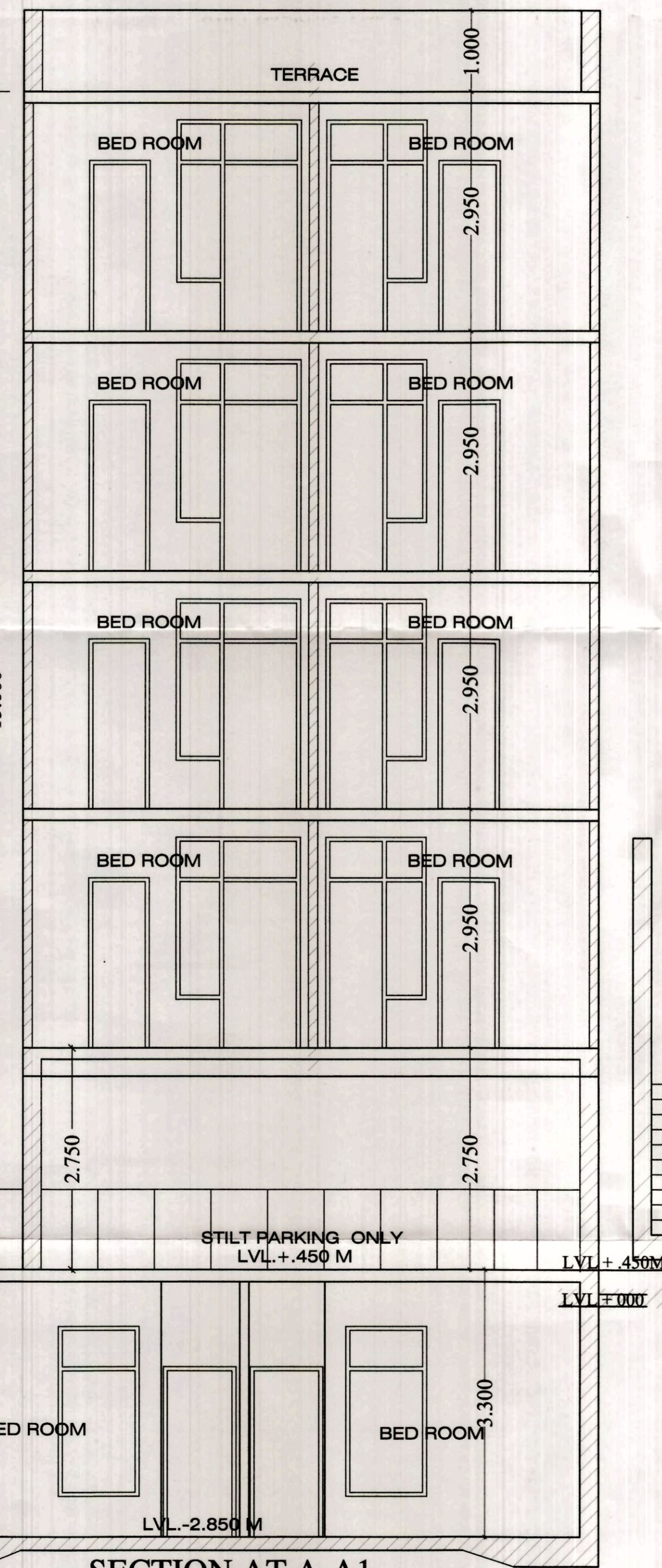
SECTION AT A-A1
