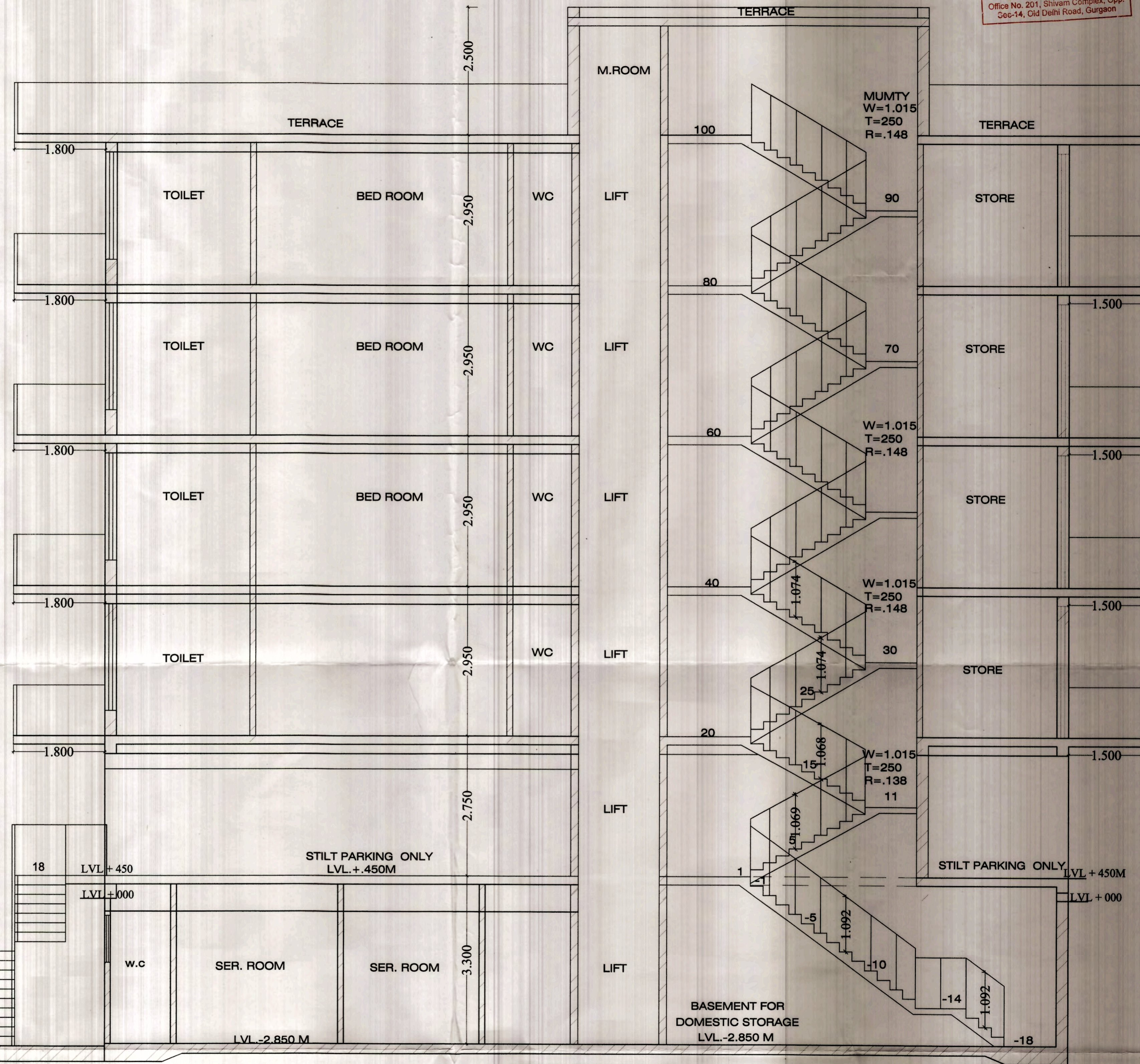
SECTION AT B-B1
