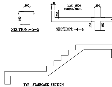
TYP. STAIRCASE SECTION
