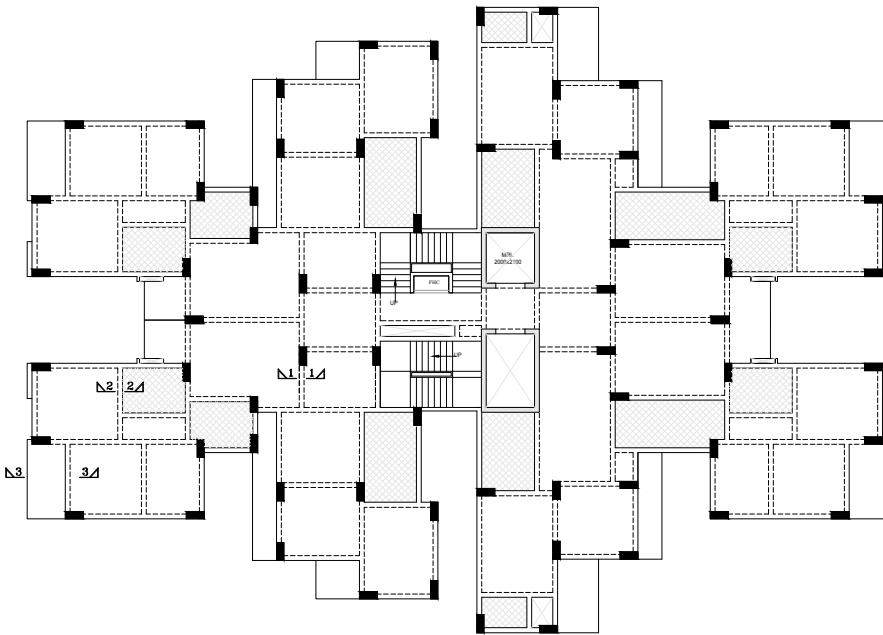
TYPICAL FLOOR LVL FRAMING PLAN TOWER G.H. I & J ( S+ 14)
