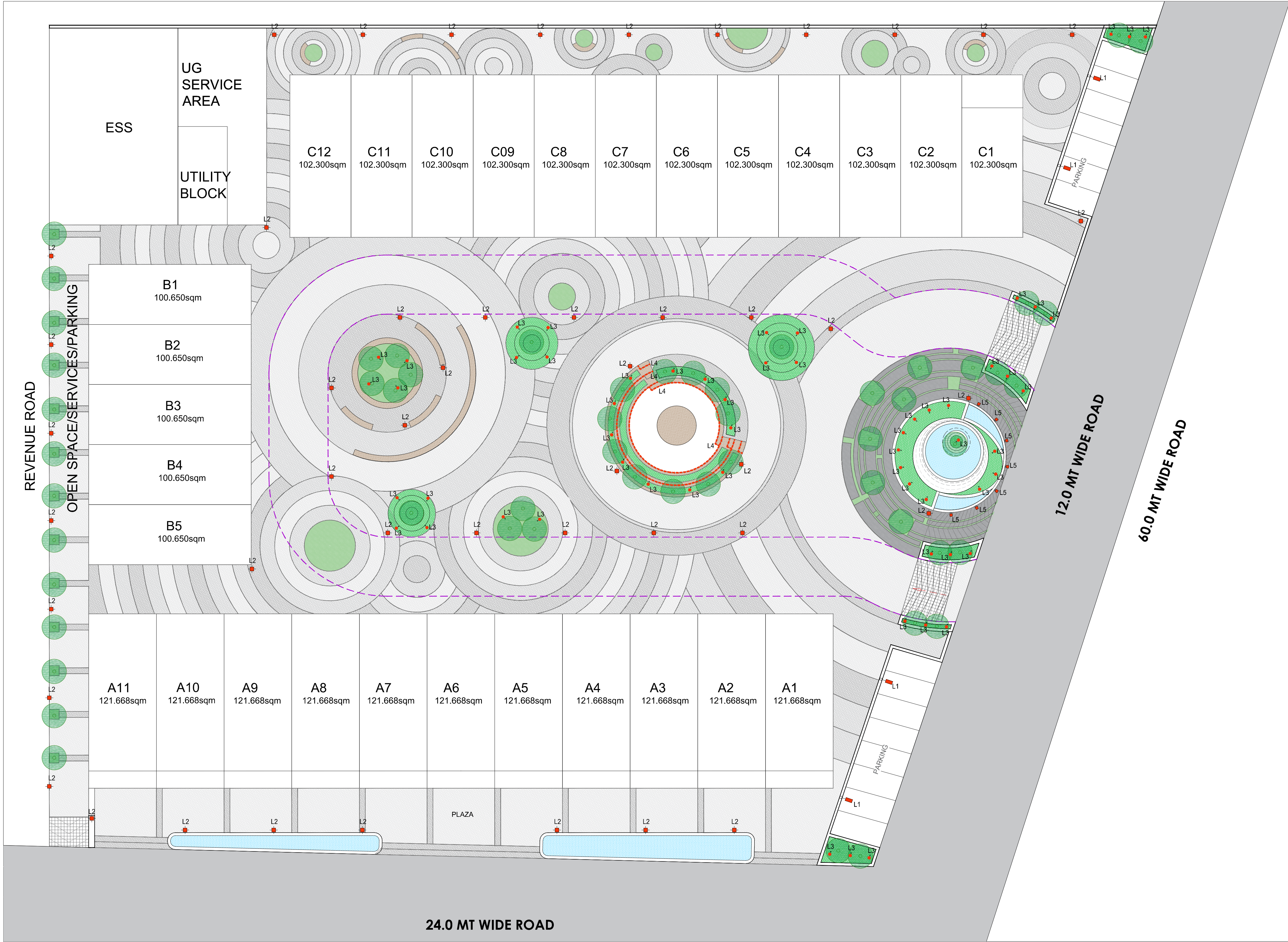
LANDSCAPE LIGHTING PLAN SCALE 1:200
