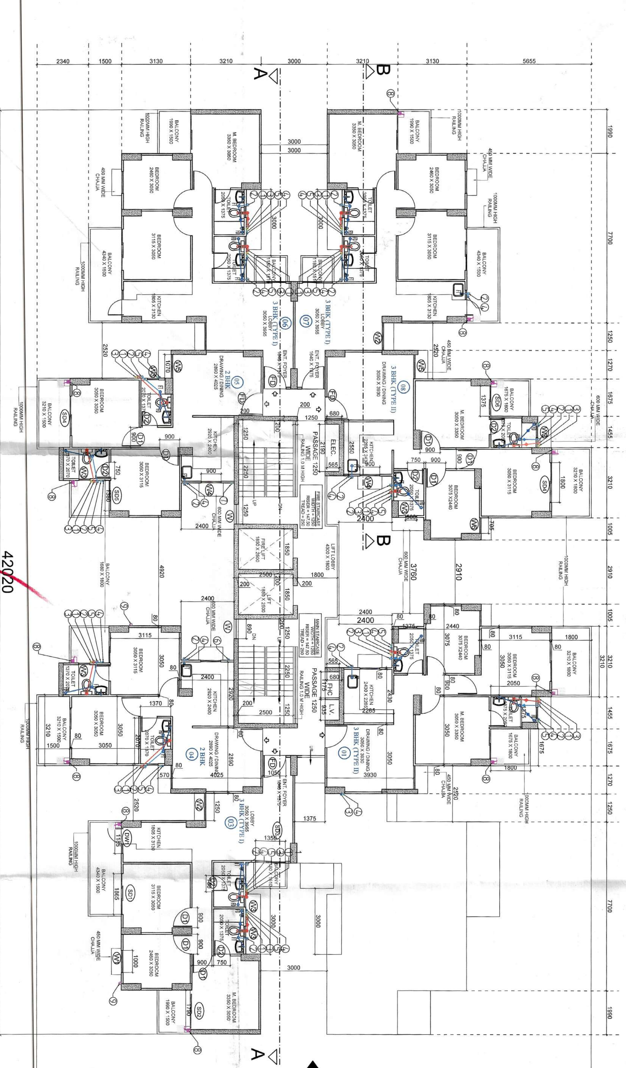
9th TO 12th FLOOR PLAN
