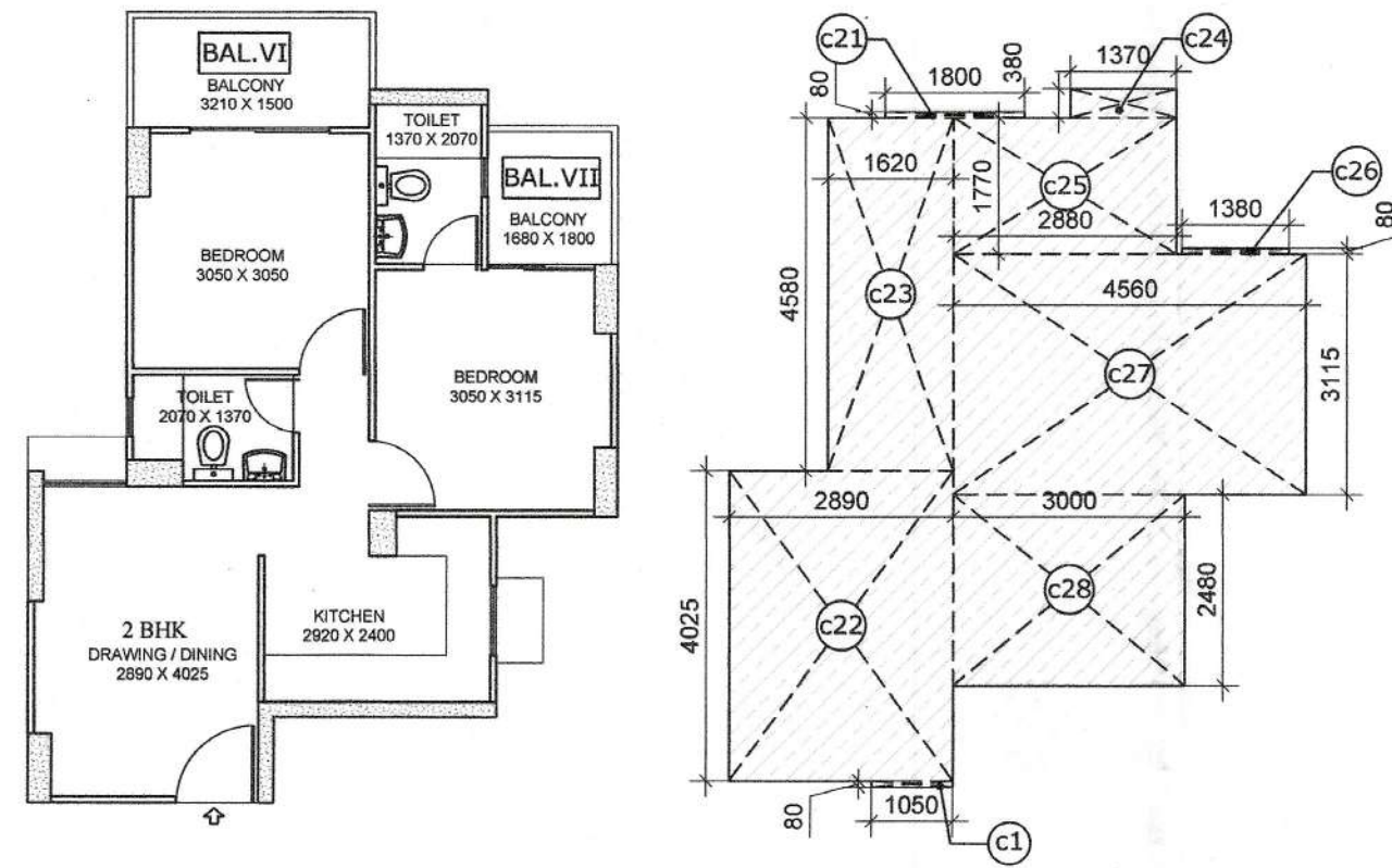
CARPET AREA DIAGRAM 2 BHK
