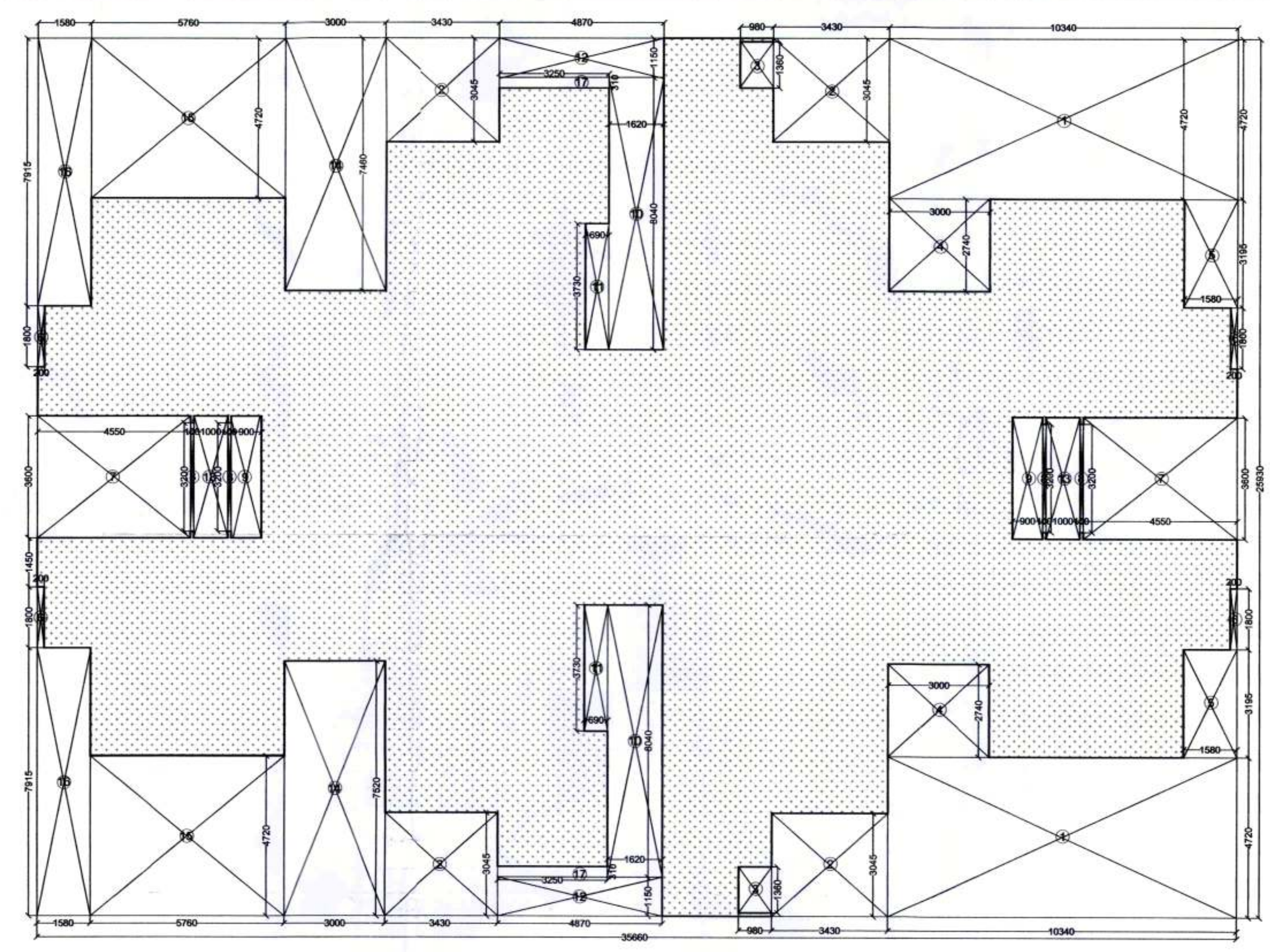
2 GROUND COVERAGE CALCULATION TOWER G,H,I,J Scale: 1:100
