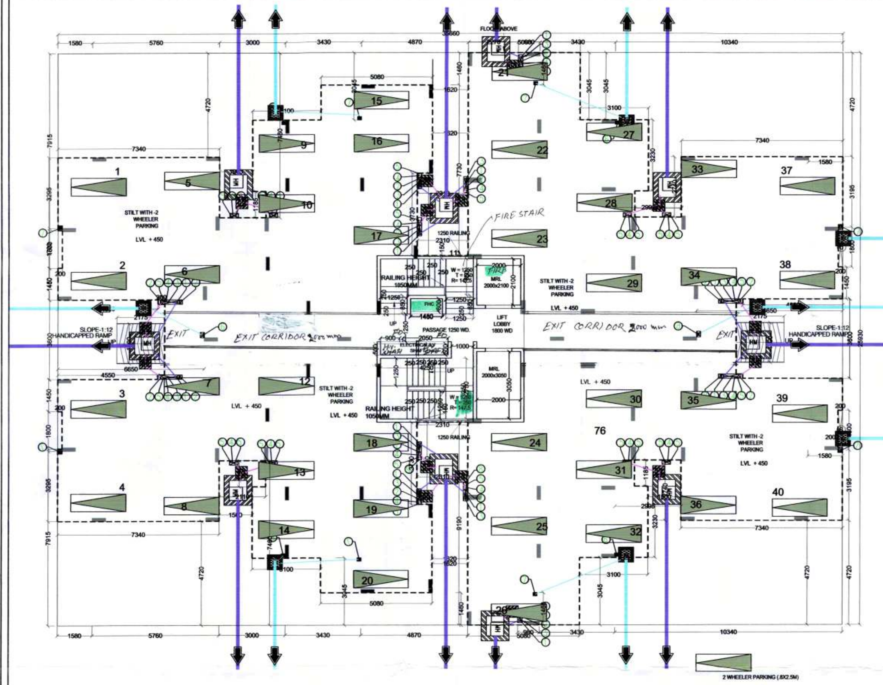
1 STILT FLOOR PLAN TOWER- G,H,I,J Scale: 1:100
