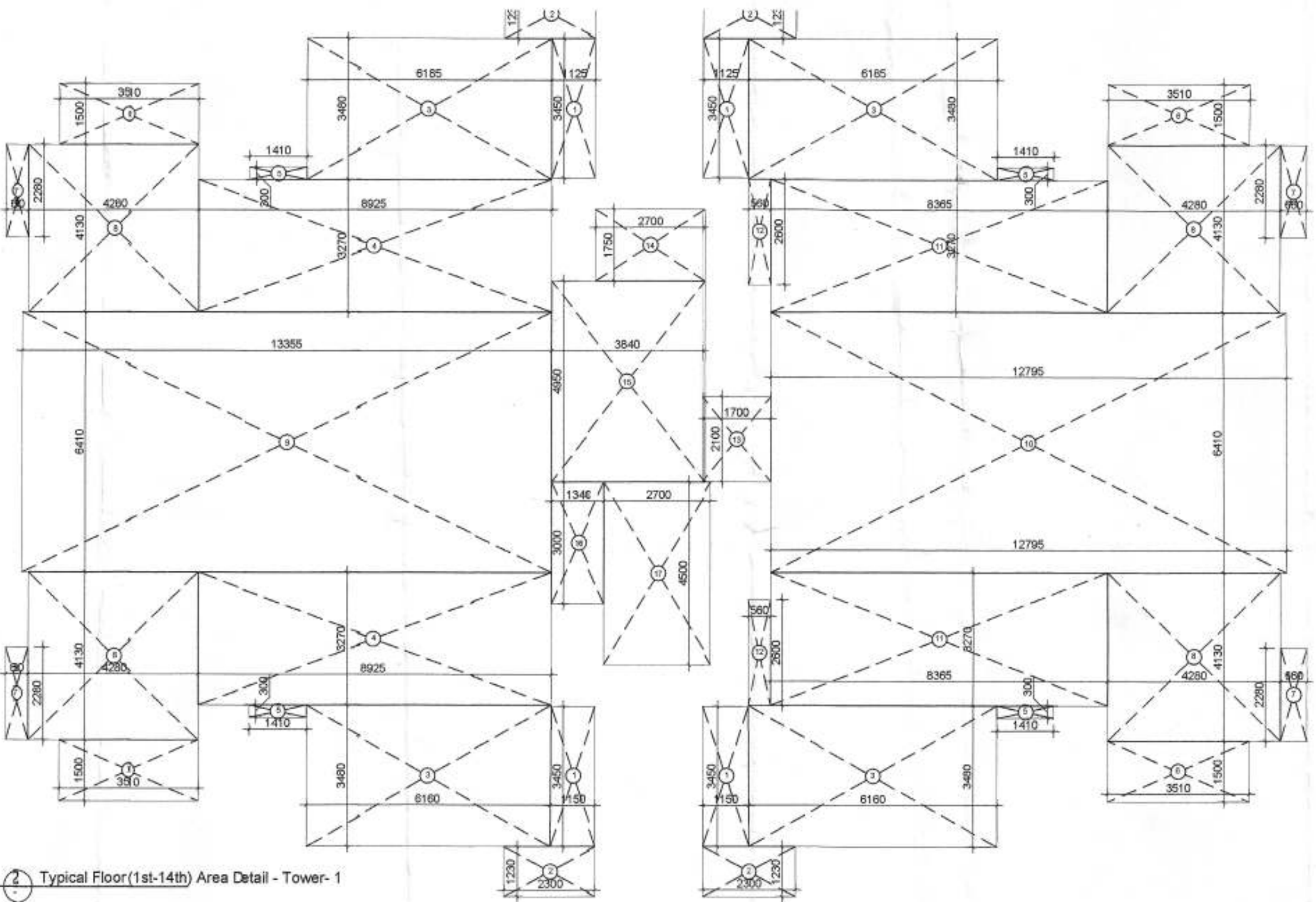
2 Typical Floor(1st-14th) Area Detail - Tower-1
