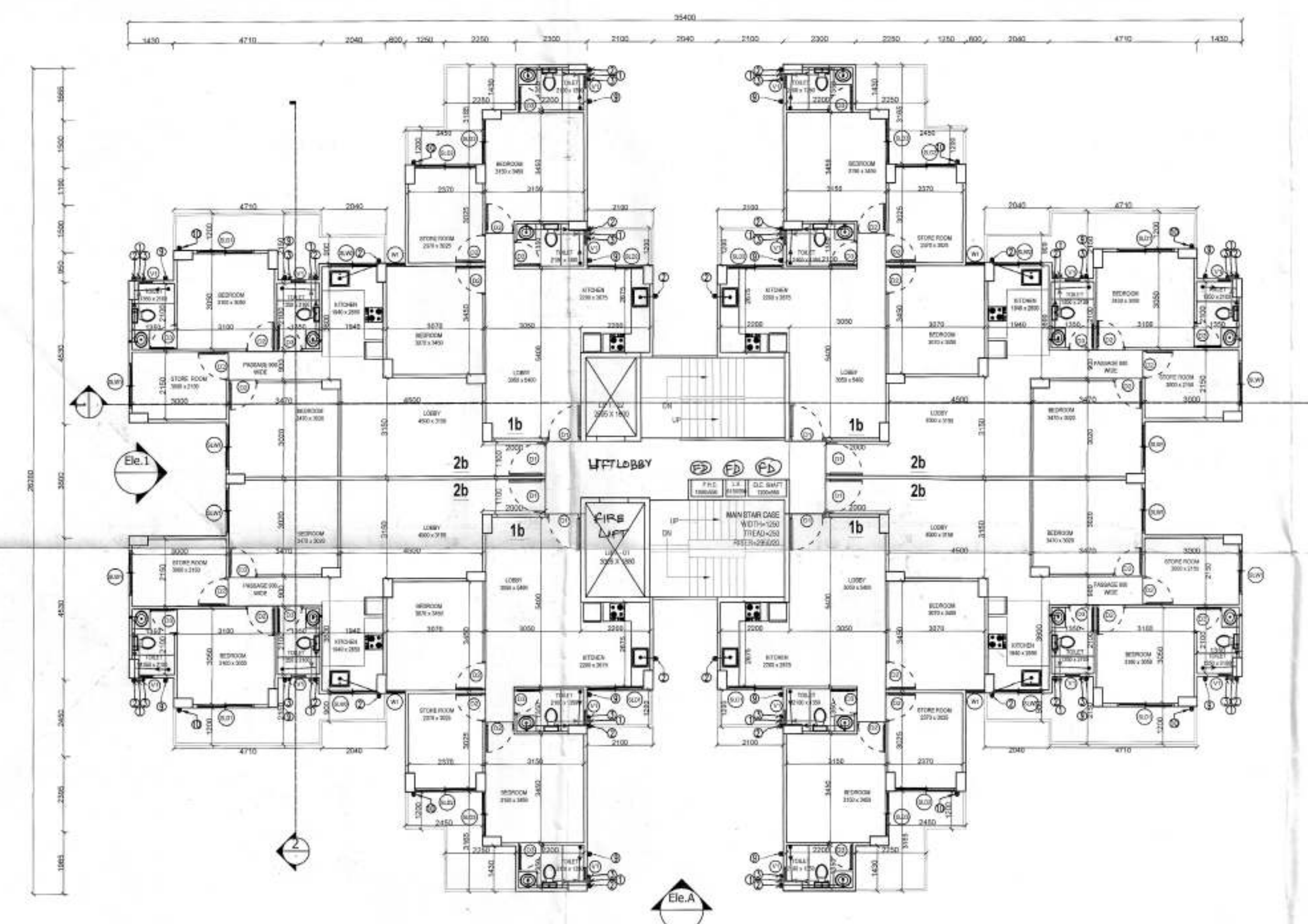
3 TYPICAL FLOOR 2nd - 12th
