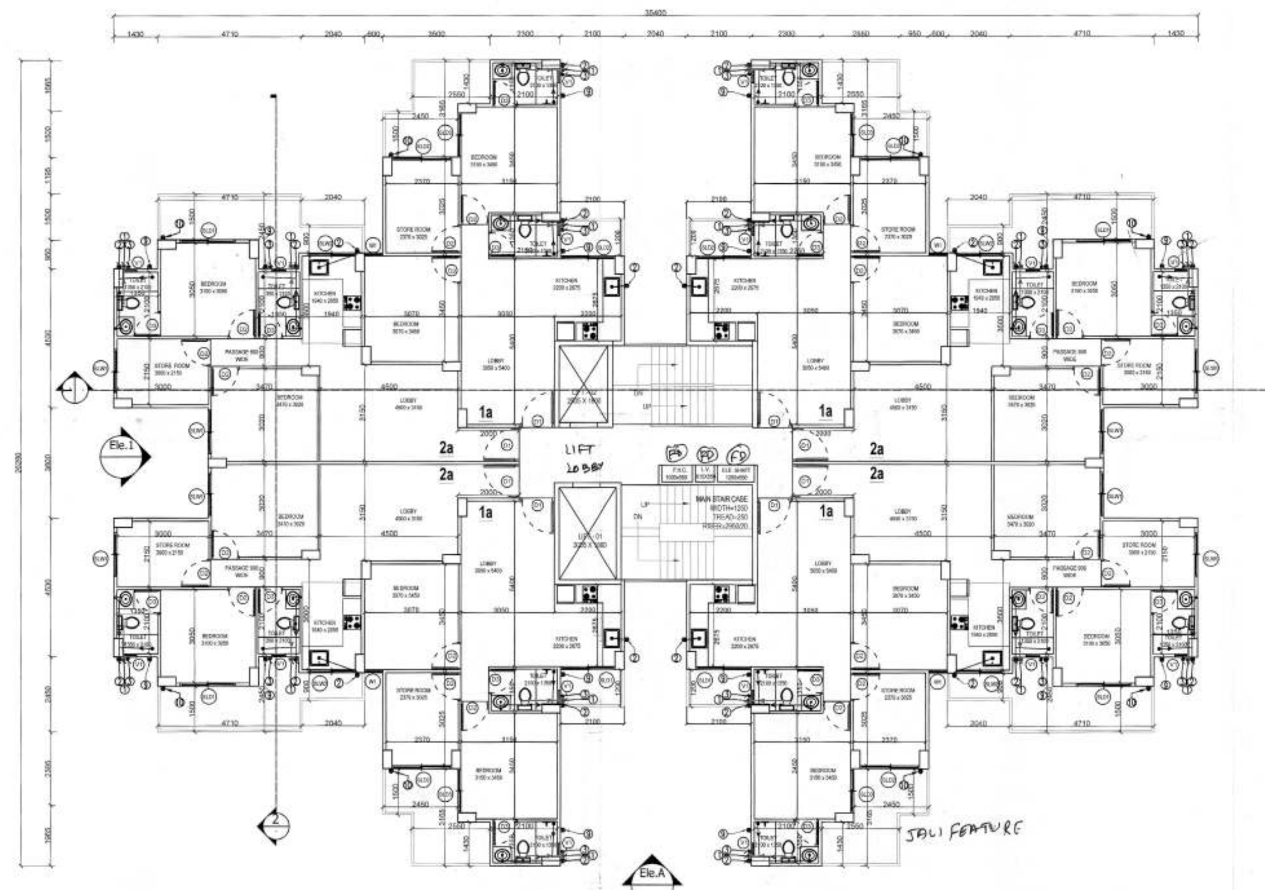
2 FIRST FLOOR PLAN TOWER-D1
