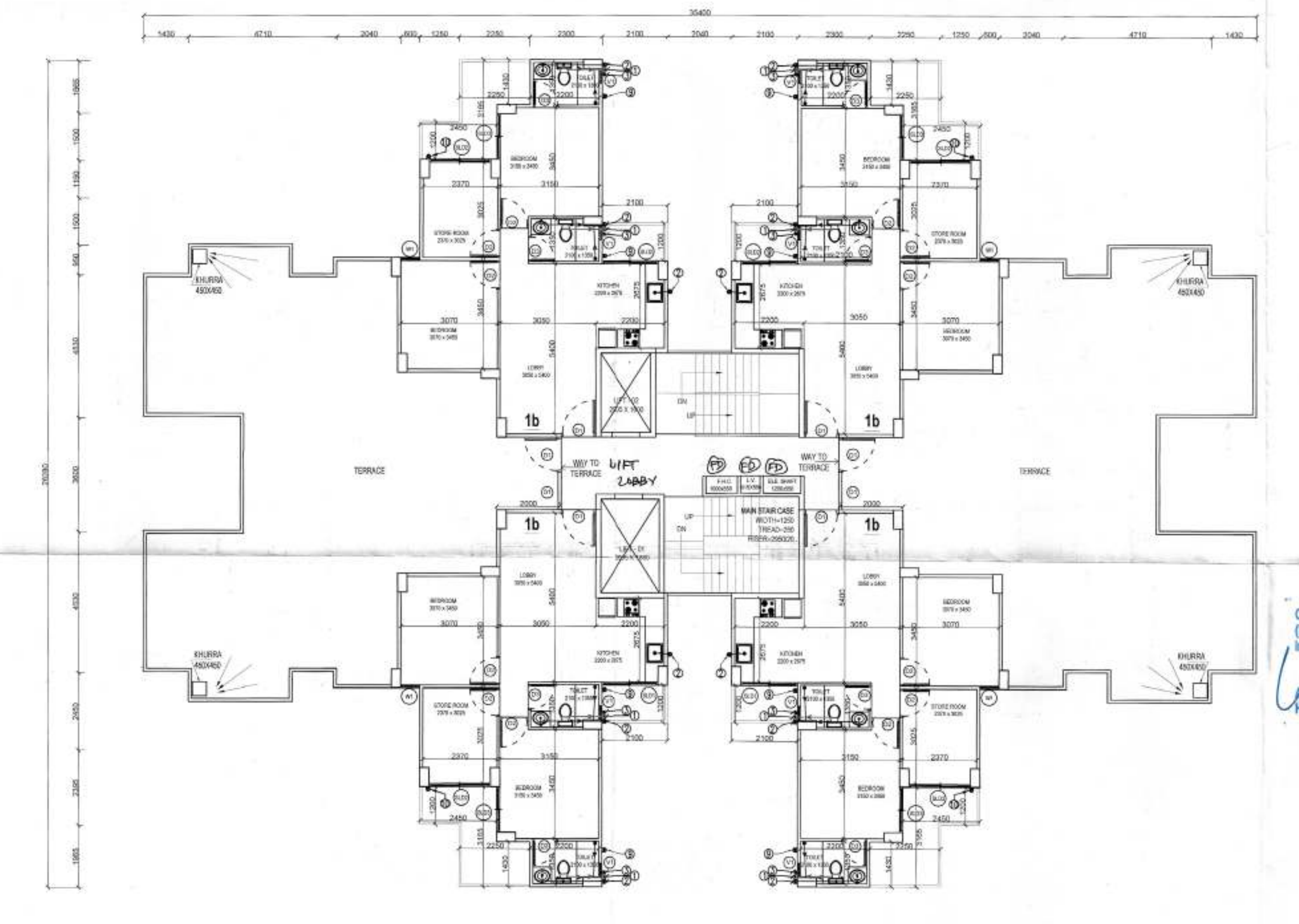
4 13th FLOOR PLAN TOWER-D1
