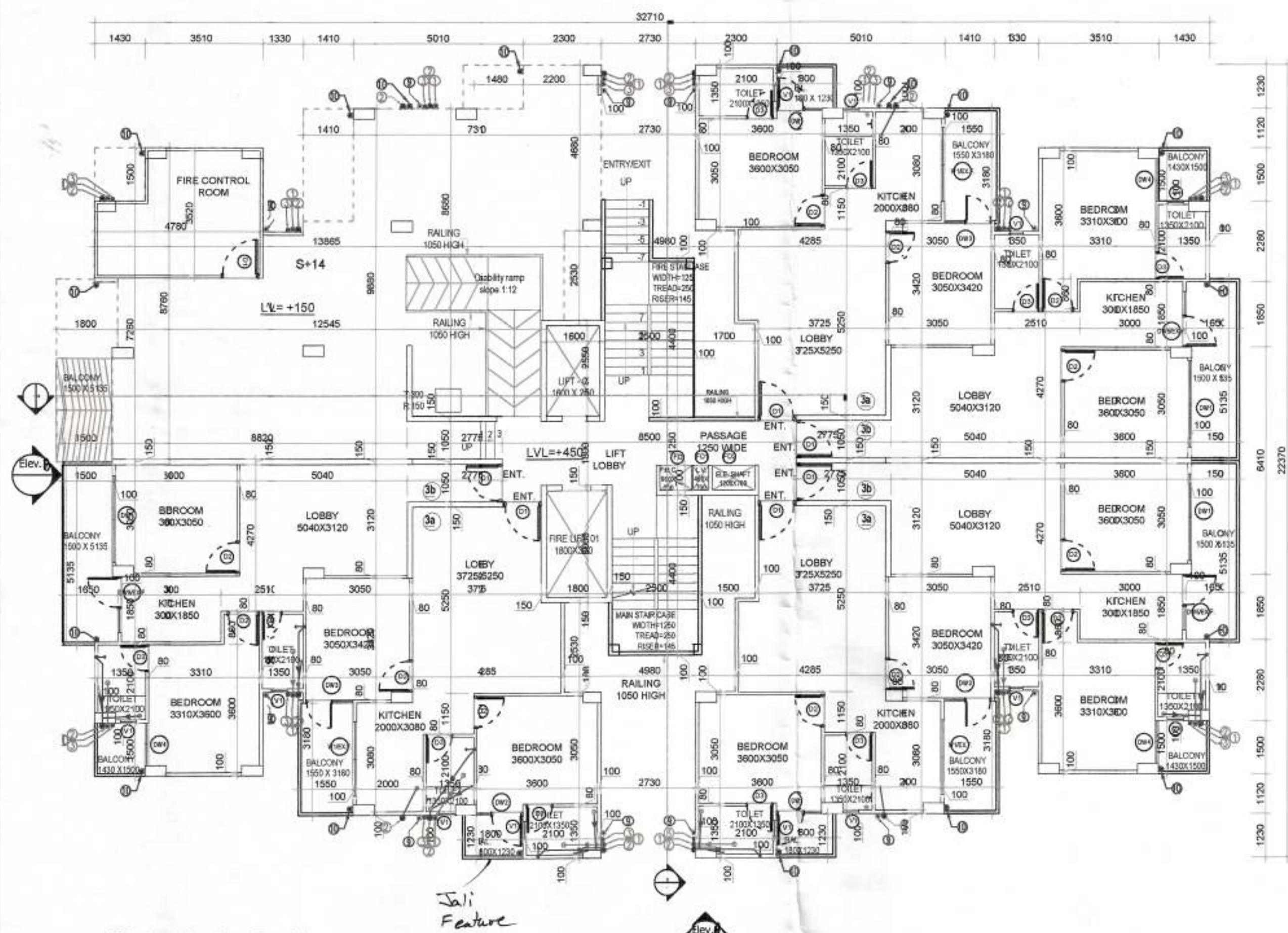
Grand floor Plan - Tower C1 TOVER C2 IS MIRROR OF TOWER C1
