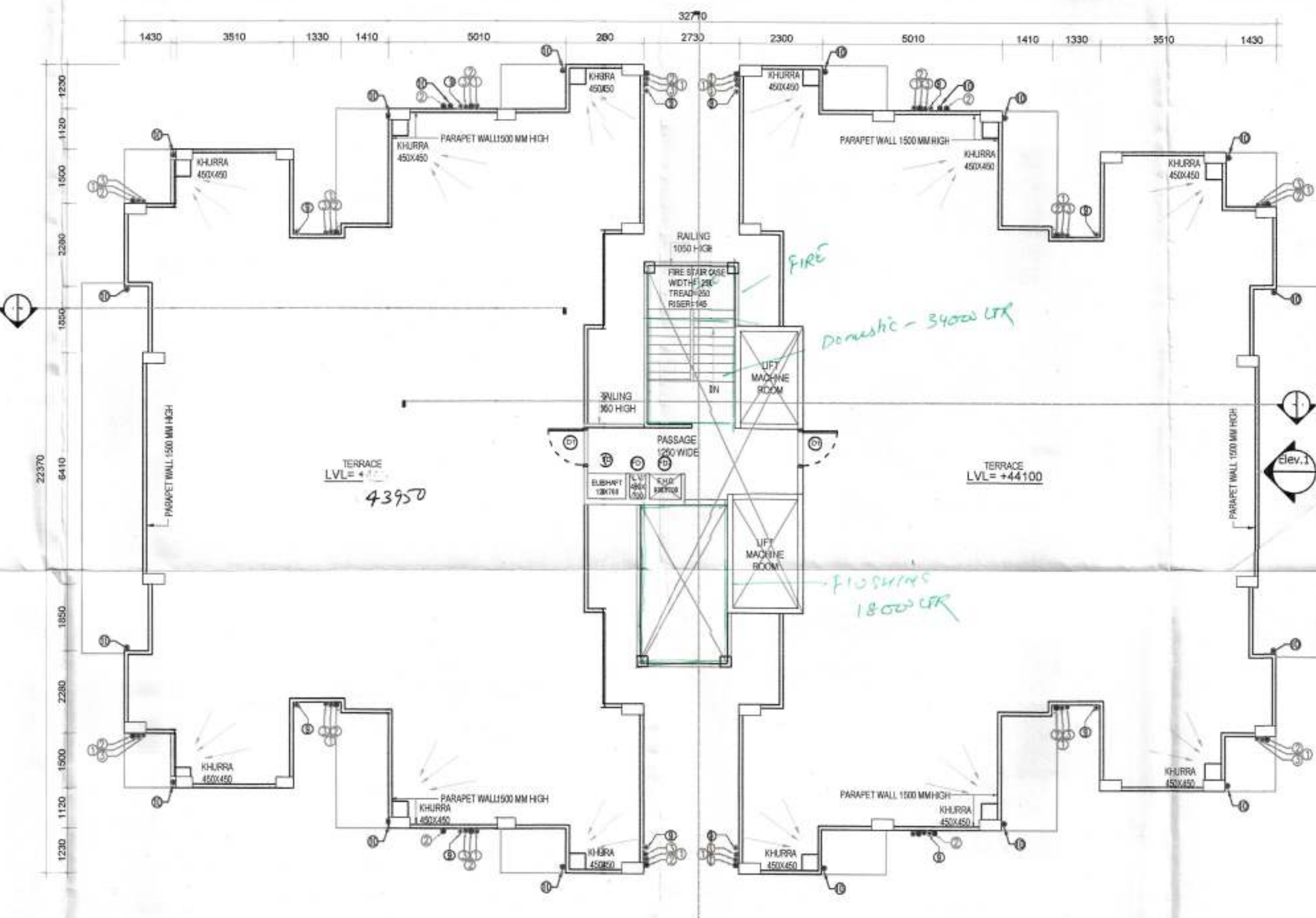
Terrace Floor- Tower C1, C2 TOVER C2 IS MIRROR OF TOWER C1
