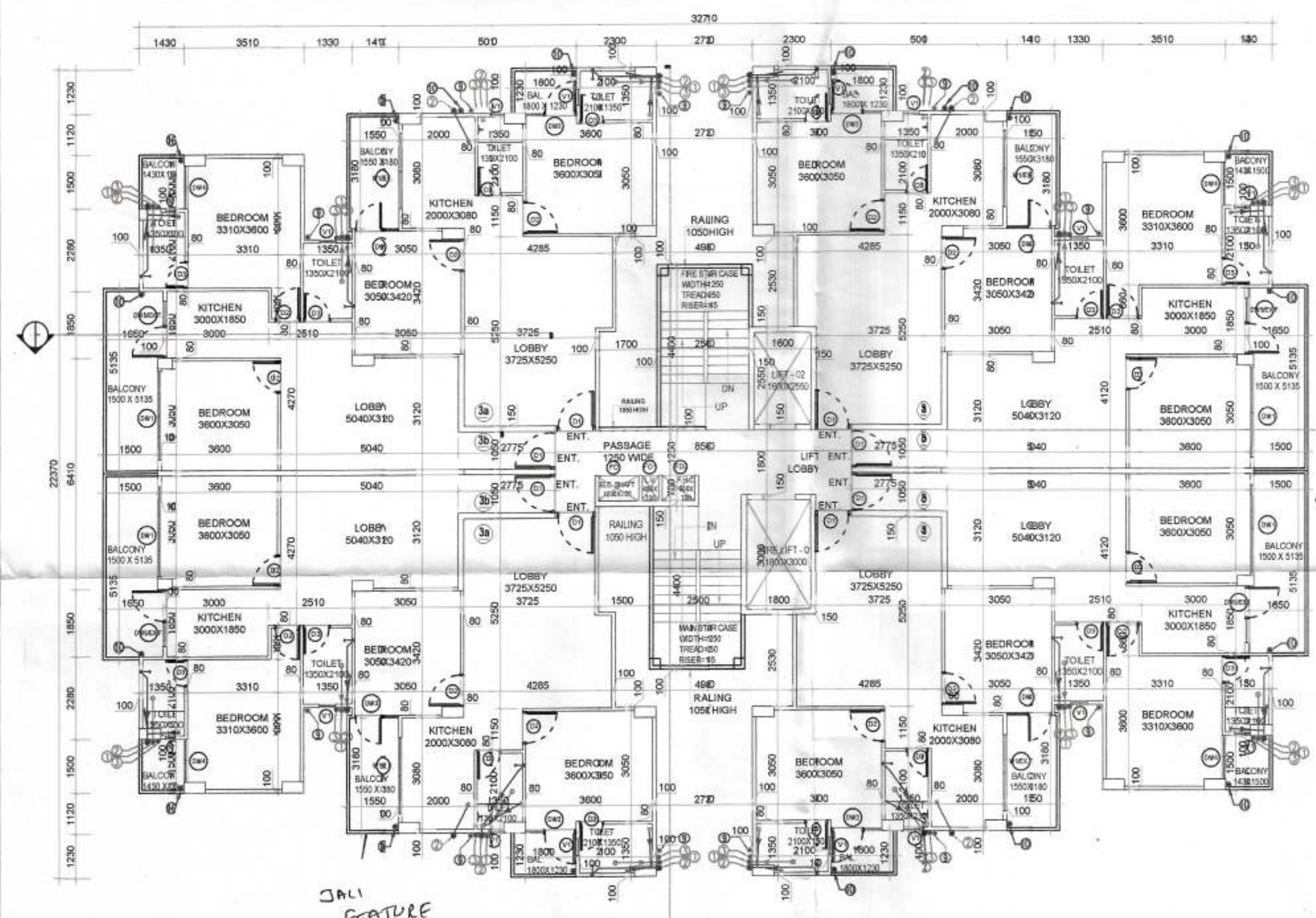
1st to 14th Floor- Tower C1, C2 TOVER C2 IS MIRROR OF TOWER C1
