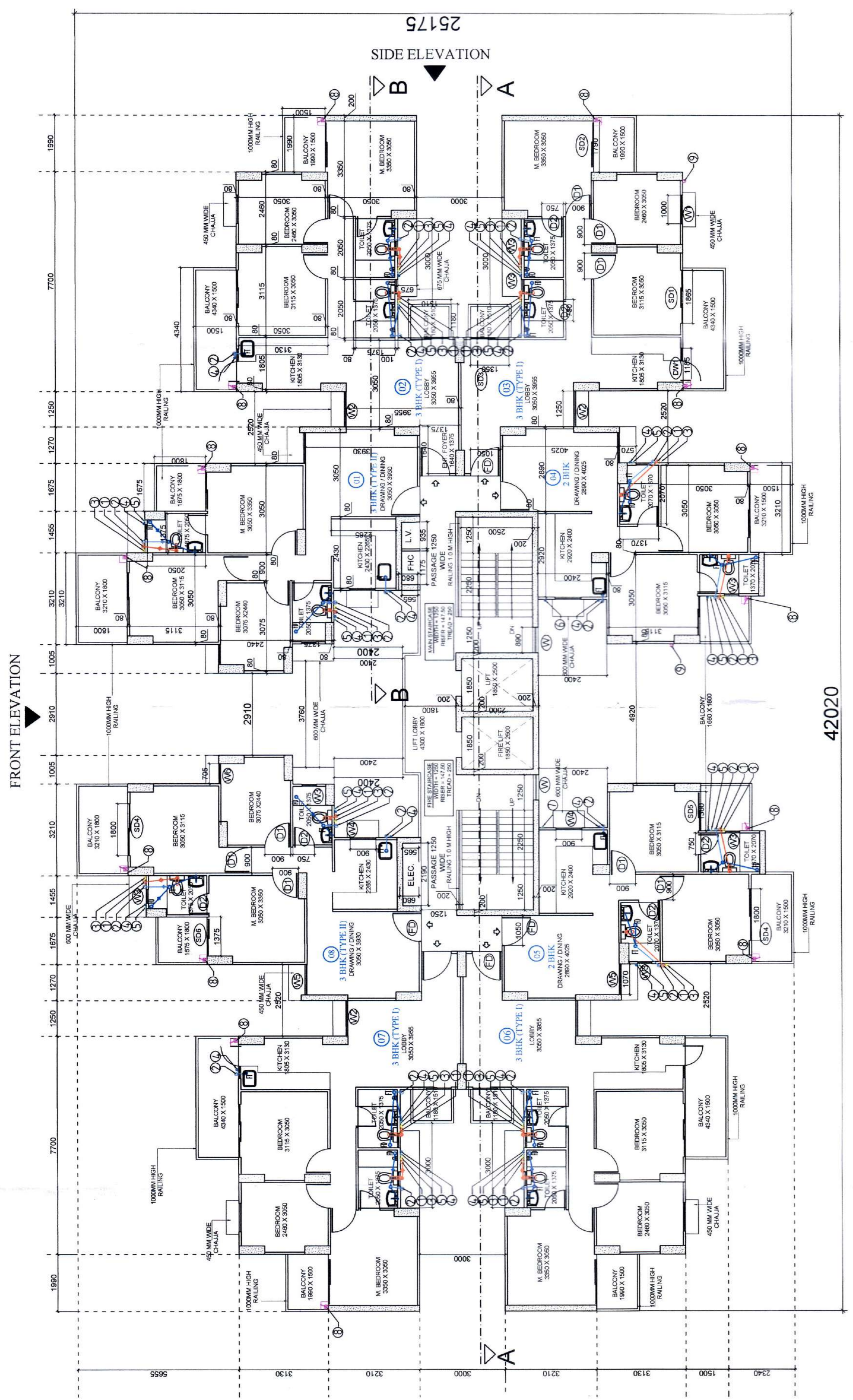
TYPICAL FLOOR PLAN (1st to 7th FLOOR)
