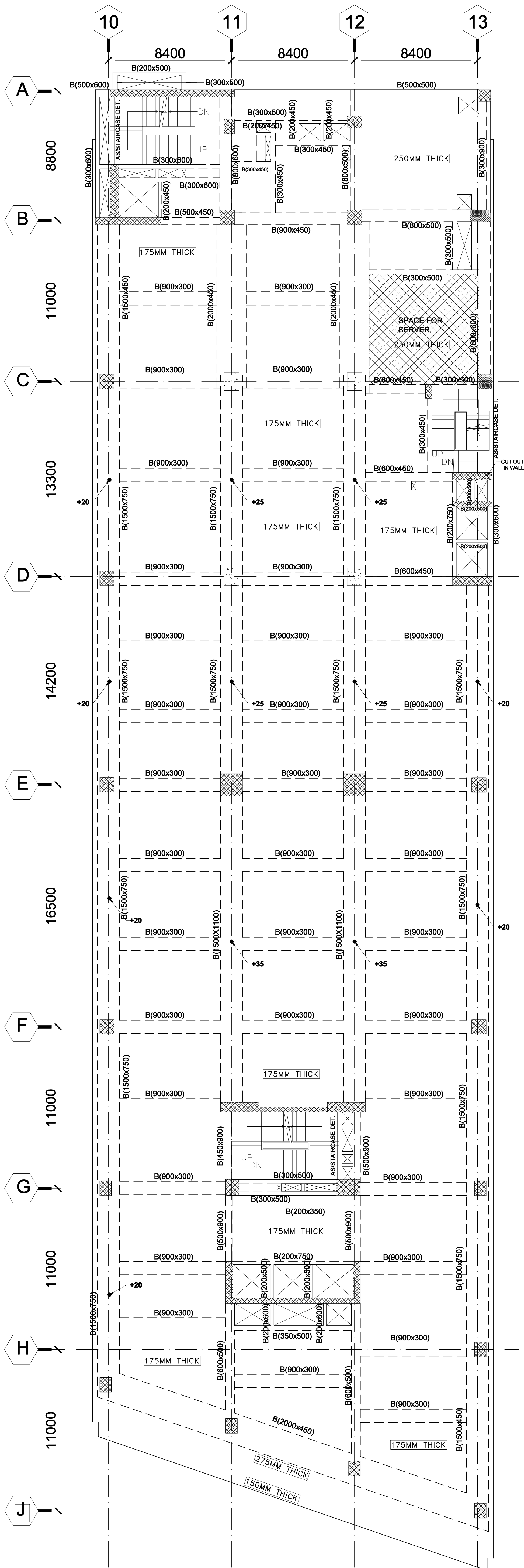
FRAMING PLAN AT TERRACE FLOOR LEVEL (TOWER-B) ALL SLABS ARE 150MM THICK UNLESS NOTED OTHERWISE
