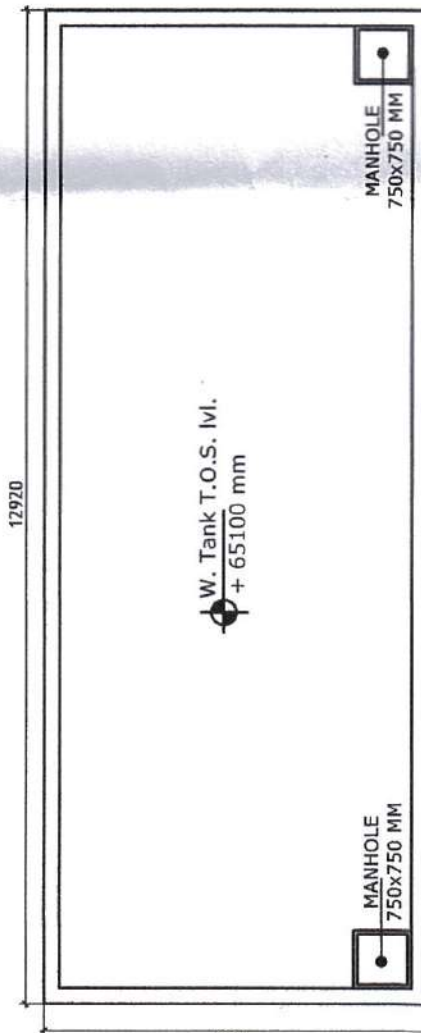
WATER TANK ROOF PLAN
